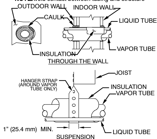
Fig. 1 - Piping Installation
