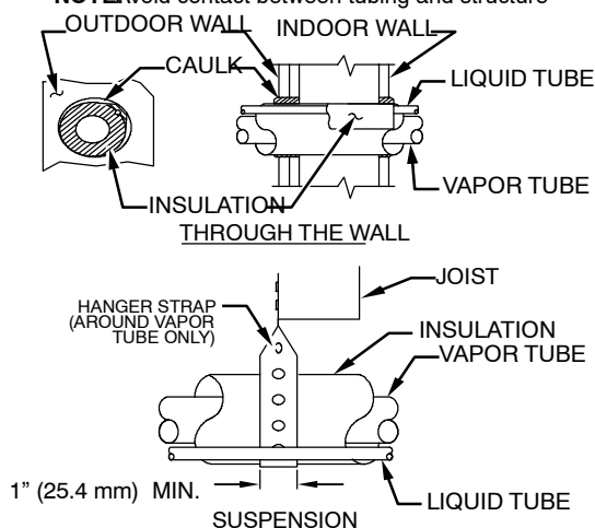
Fig. 1 - Piping Installation
