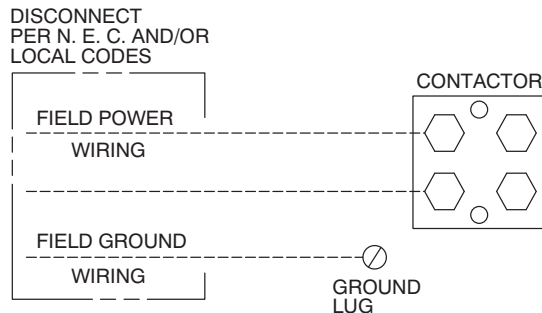
Fig. 6 - Line Connections
