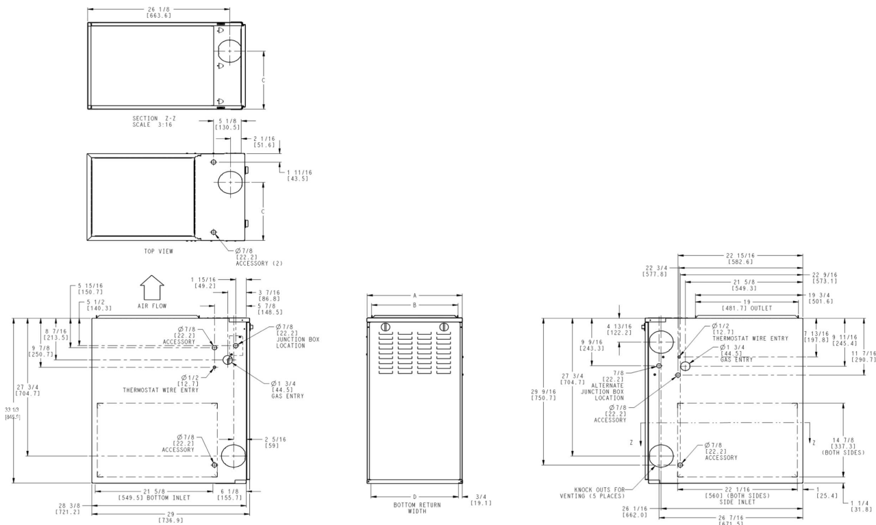
Fig. 1 – Dimensional Drawing
