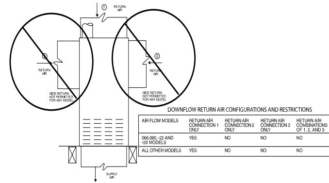
Fig. 18 – Downflow Return Air Configurations and Restrictions A02163
