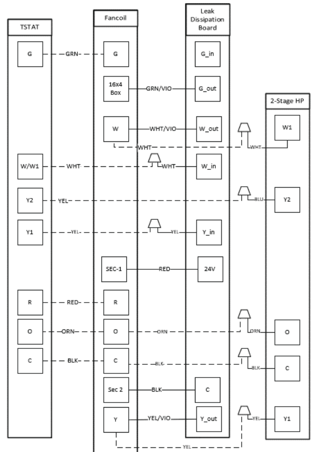
Fig. 10 – Thermidistat Wiring with Fan Coil and 2-Stage HP
