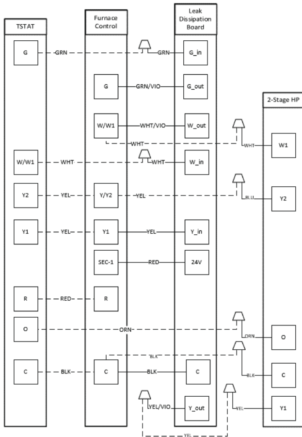
Fig. 9 – Thermidistat with Variable Speed Furnace and 2-Stage Heat Pump
