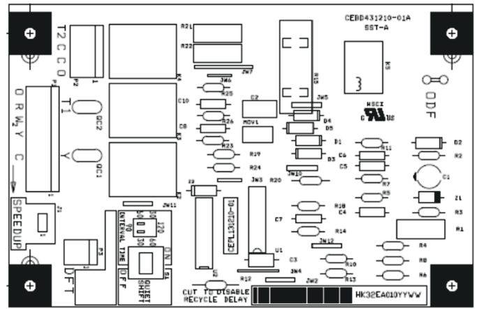
Fig. 11 – Defrost Control
