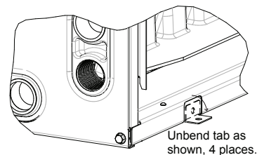
Fig. 6 - Horizontal Left Installation
