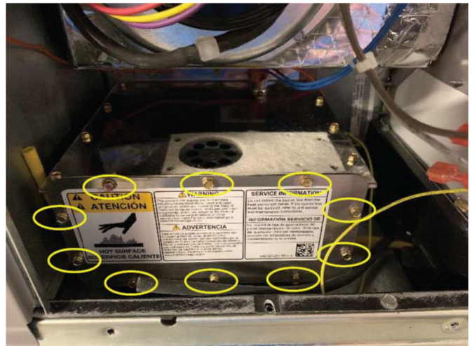
Fig. 4 – Removing Burner Box Cover Screws
