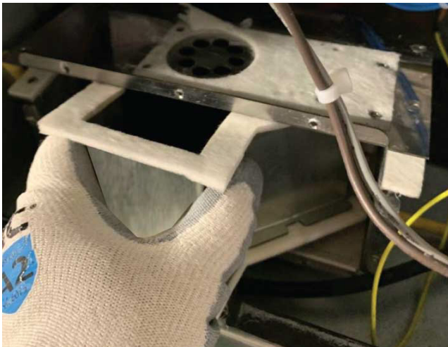
Fig. 8 – Removing Baffle from Burner Box
