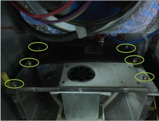
Fig. 6 – Removing Screws from Top Cover of Burner Box
