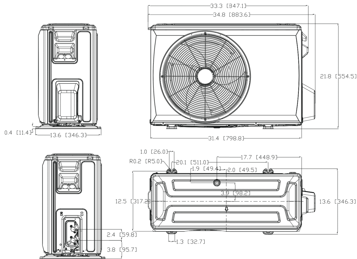
Fig. 4 —Dimensions (24k)
