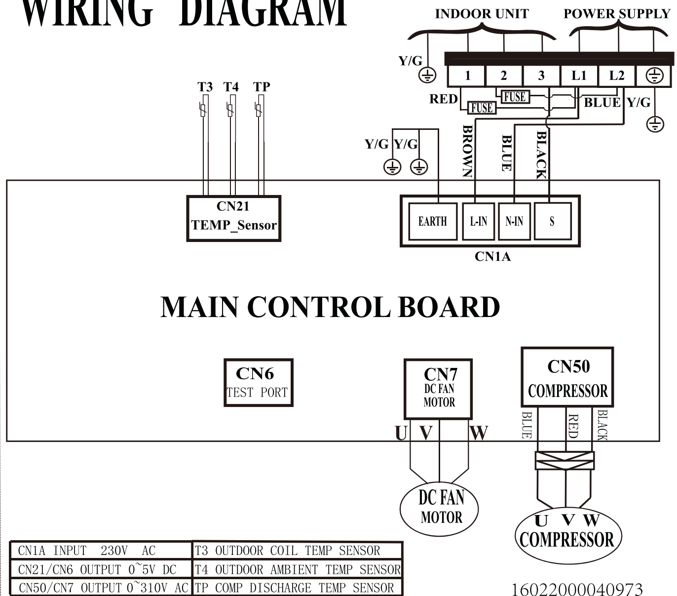
Fig. 9 — Wiring Diagram Sizes - 9-18K (208-230V)
