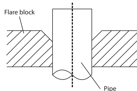
Fig. 12 — Flare Block
