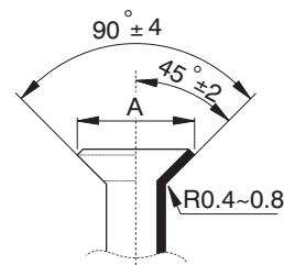
Fig. 13 — Flare Shape
