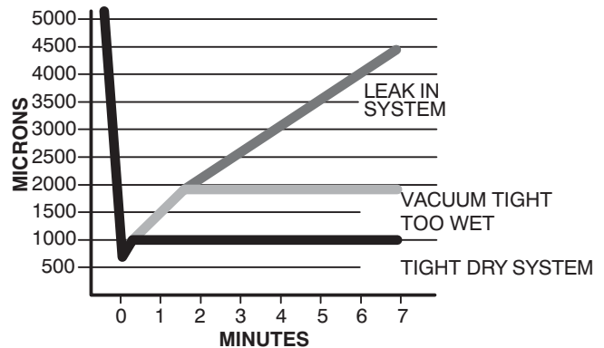
Fig. 35 —Deep Vacuum Graph
