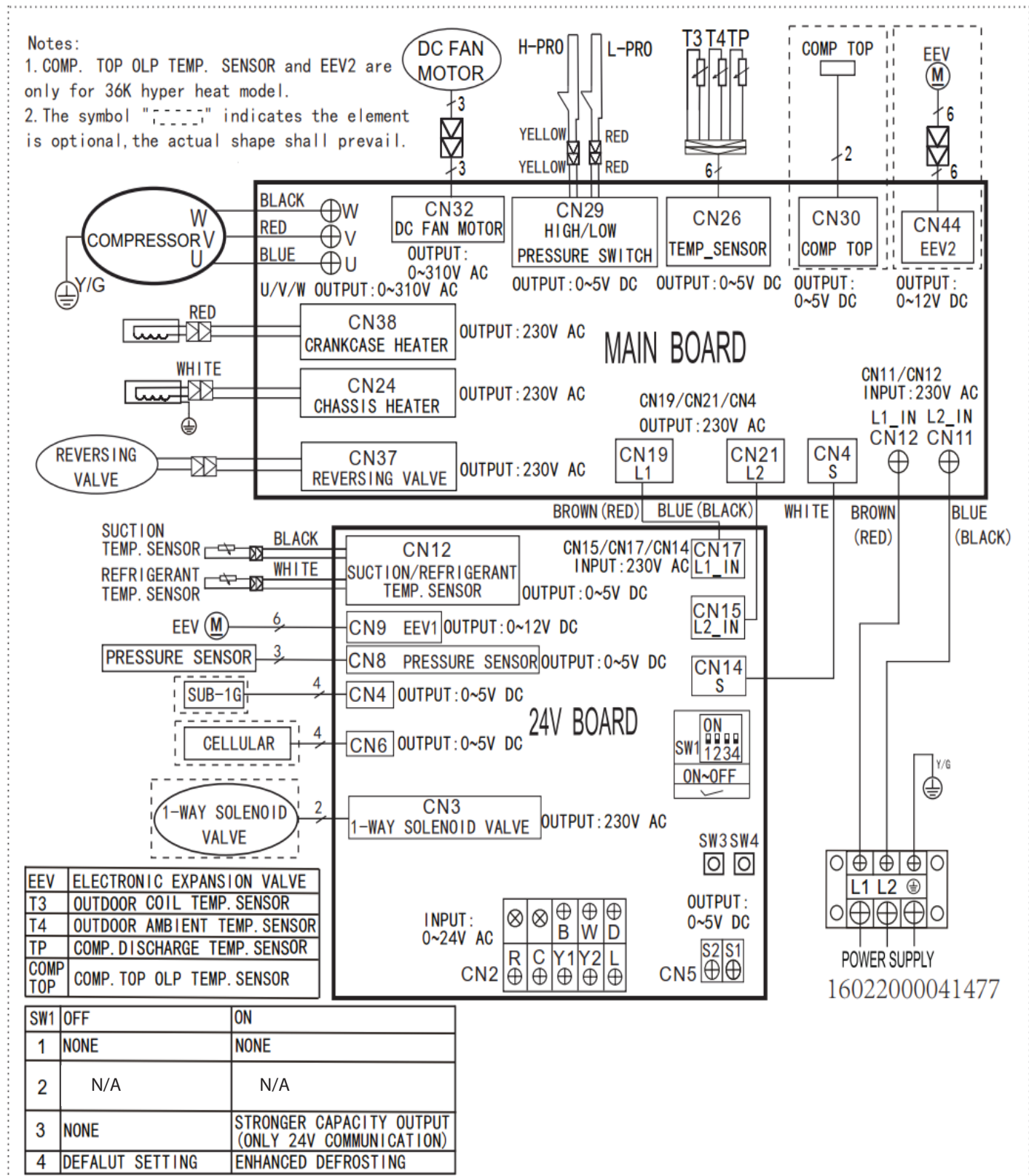
Fig. 28 — Sizes 36K and 48K
