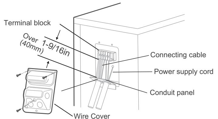
Fig. 23 —Outdoor Unit Wiring
