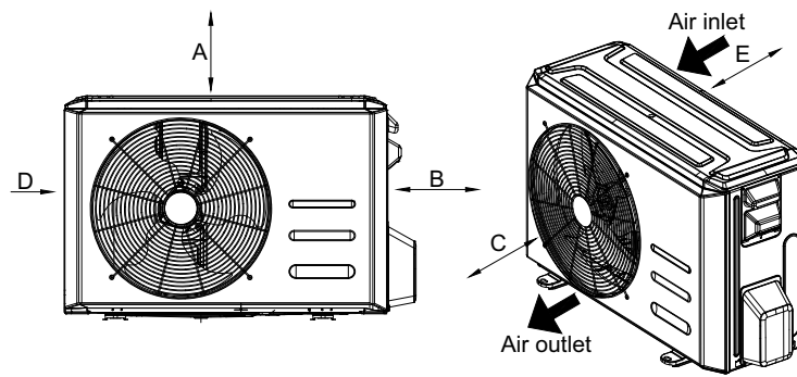
Fig. 17 – Clearances
