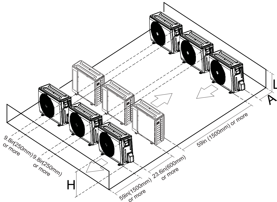
Fig. 18 – Clearance for Multiple Units
