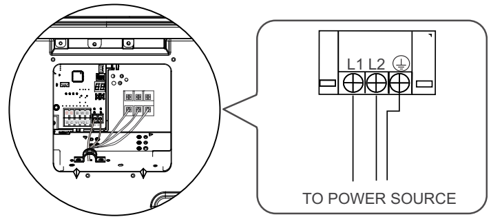
Fig. 22 —Connect Fork Terminals to Terminals (Sizes 30K-60K)
