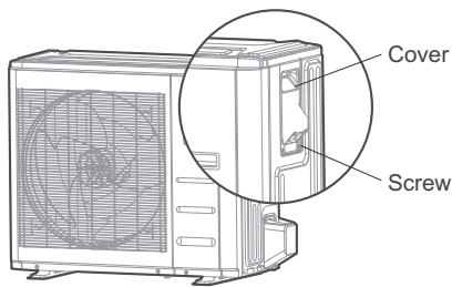
Fig. 20 —Remove Electrical Cover
