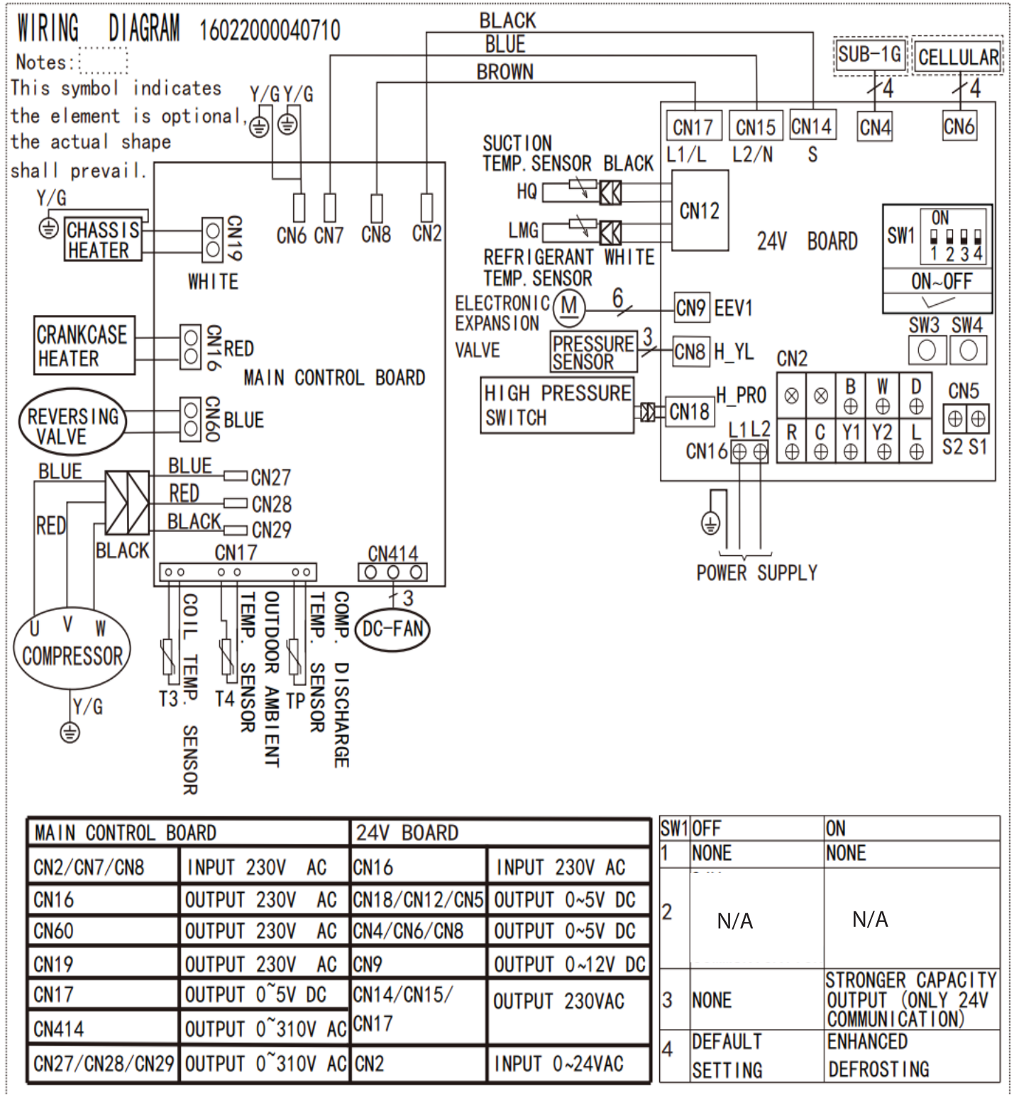
Fig. 26 — Sizes 18K and 24K
