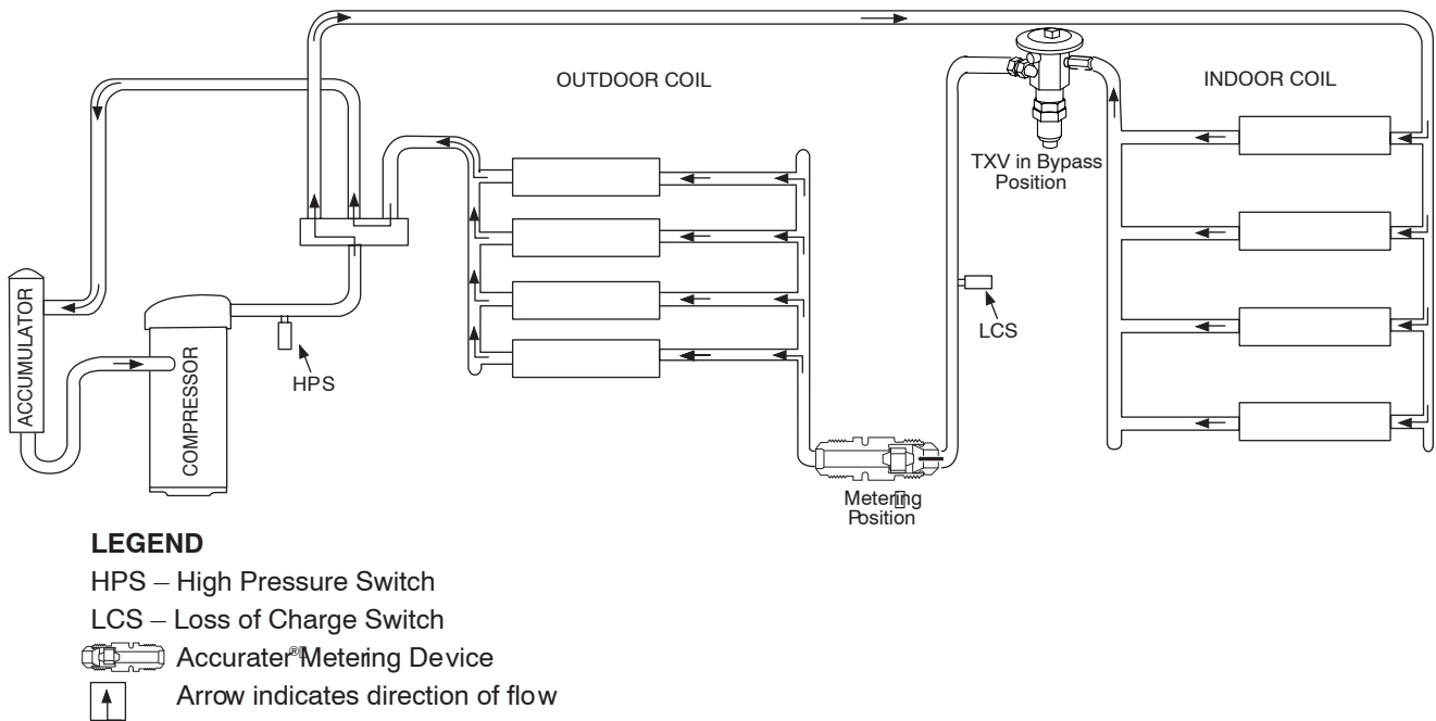
Fig. 30 - Typical Heat Pump Operation, Heating Mode
