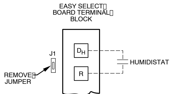
Fig. 15 - Humidistat Wiring for De-Humidify Mode - 48XZ
