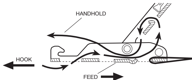
Fig. 7 - How to Loop Rigging Belt
