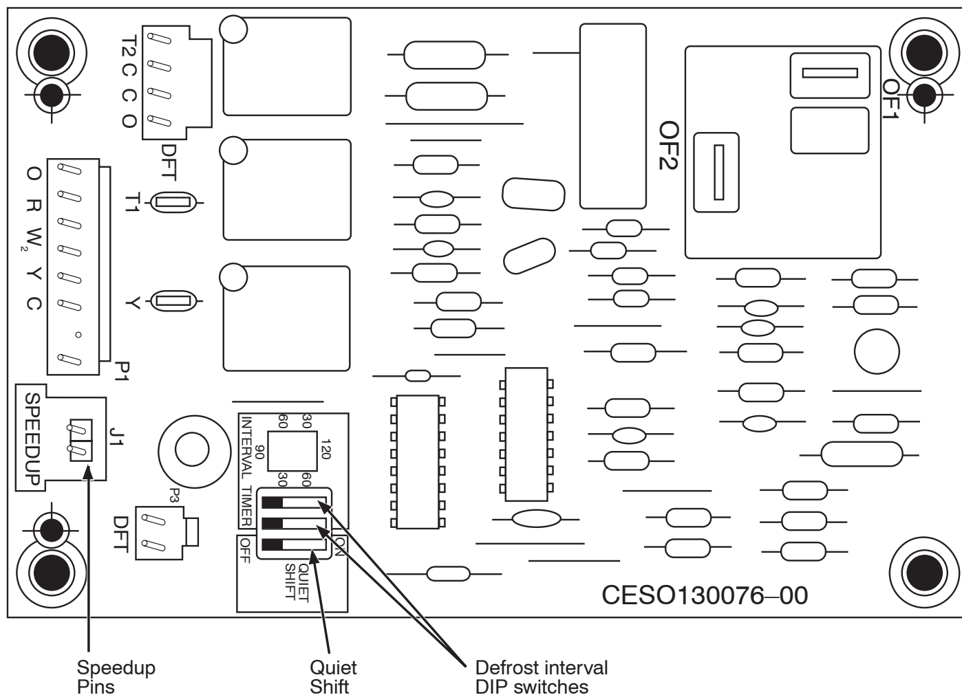
Fig. 27 - Defrost Control
