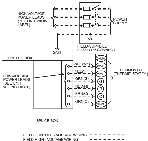
Fig. 12 - High and Control-Voltage Connections
