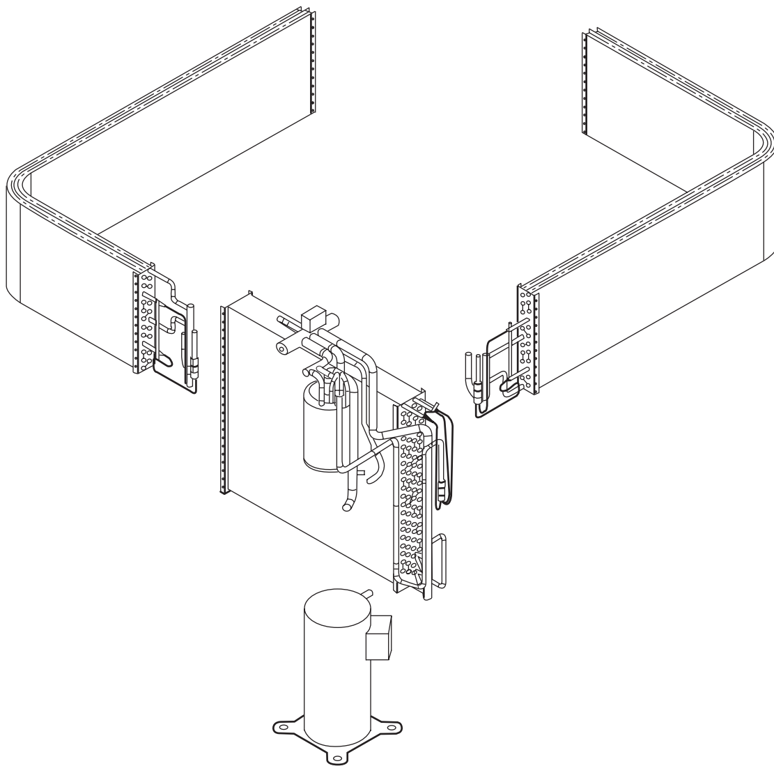
Fig. 28 - Refrigerant Circuit
