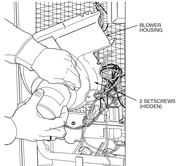
Fig. 24 - Removal of Motor and Blower Wheel
