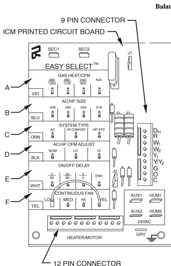
Fig. 13 - Detail of SPP Printed-Circuit Board
