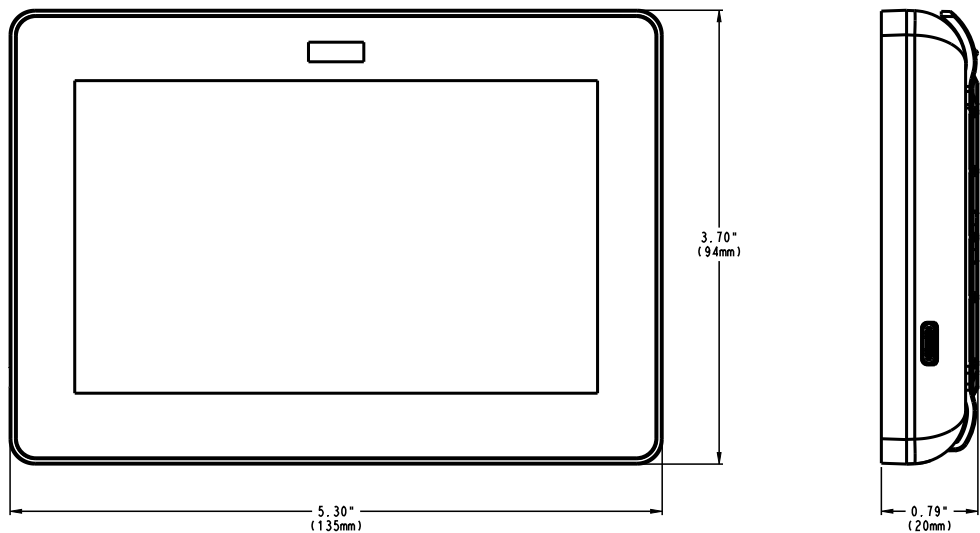
Fig. 1 – Unit Dimensions
