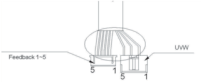
Fig. 34 —Outdoor DC Fan Motor (DC motor that controls the chip on the PCB)
