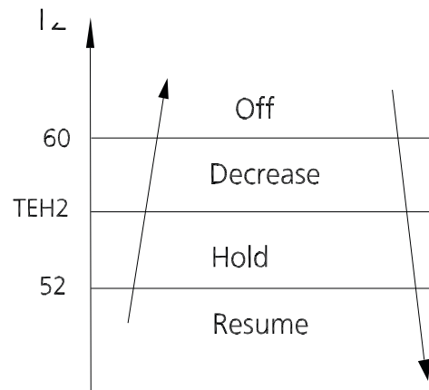
Fig. 24 —Evaporator Coil Temperature Protection
