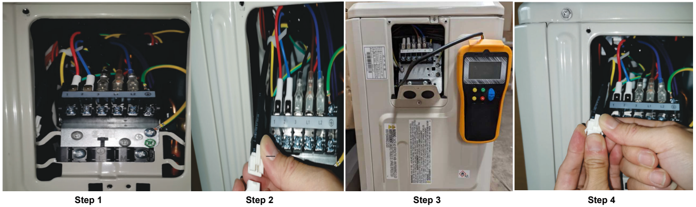
Fig. 28 —Inverter Test Tool Maintenance
