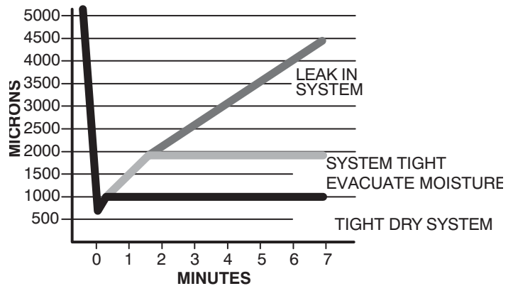
Fig. 13 —Deep Vacuum Graph
