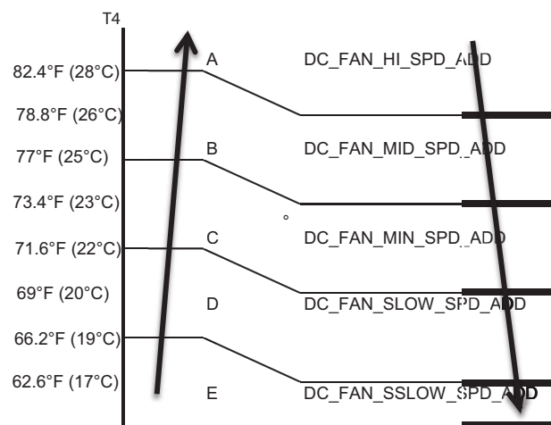
Fig. 16 —Outdoor Fan Running Rules
