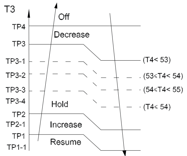
Fig. 19 —Compressor Temperature Protection
