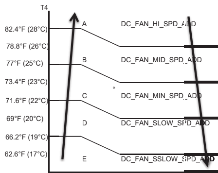
Fig. 21 —Outdoor Fan Running Rules
