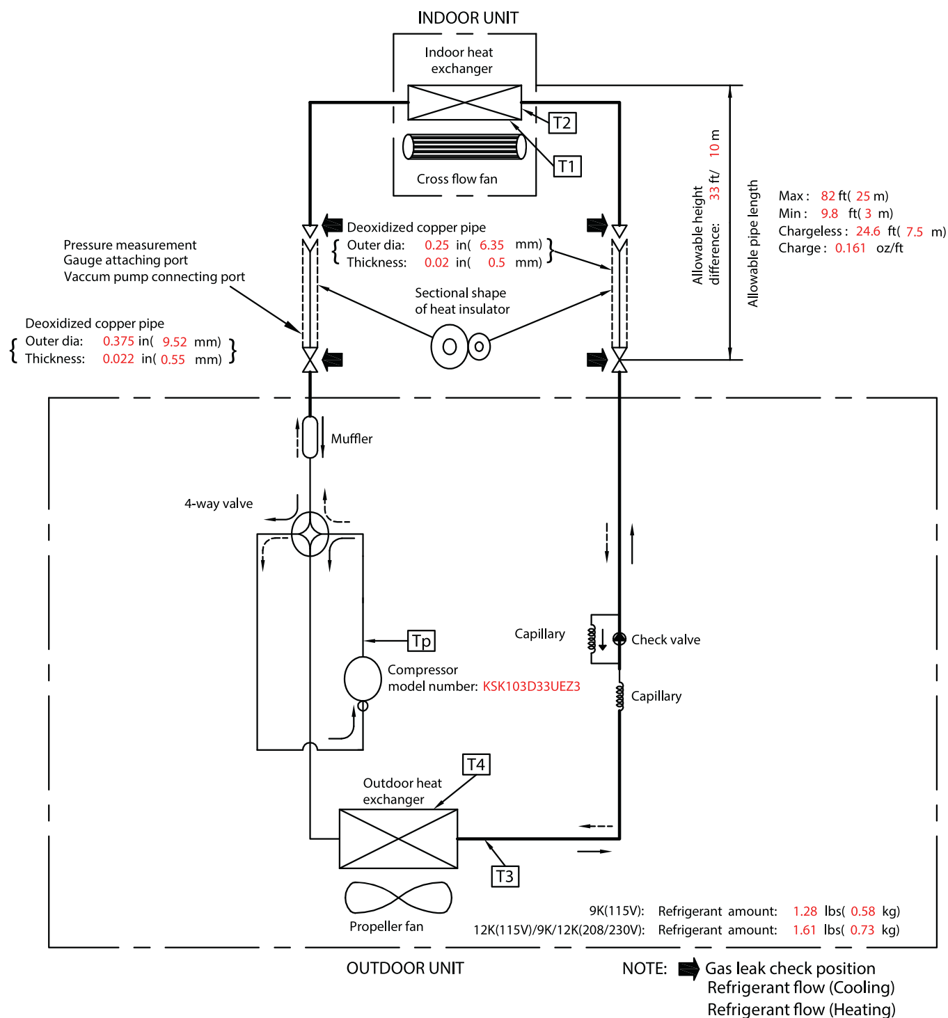
Fig. 8 —9-12K (115V) and 9-12K (208/230V)
