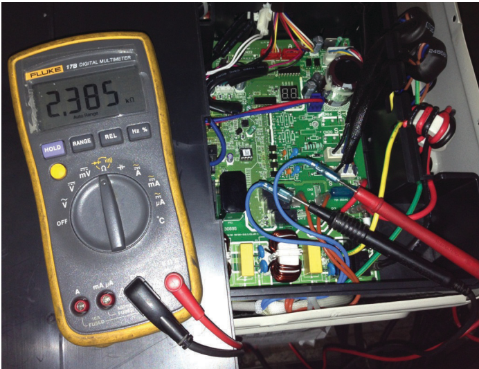
Fig. 41 —Use a Digital Tester to Measure Resistance
