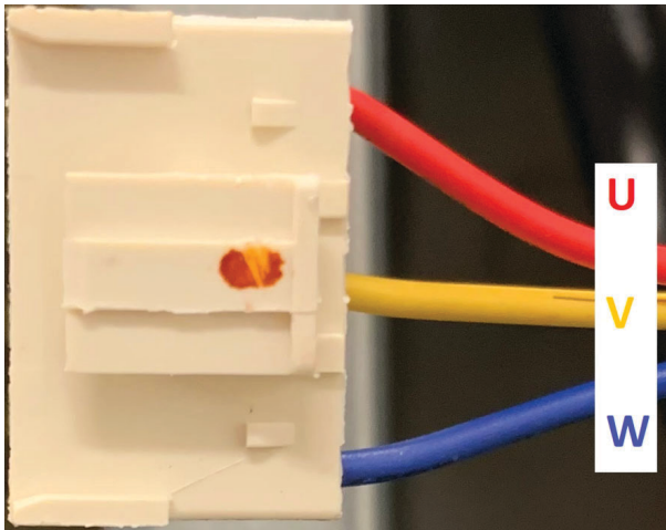
Fig. 35 —U-V-W Plug End
