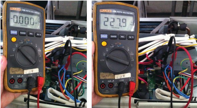
Fig. 40 —Measure the Voltage
