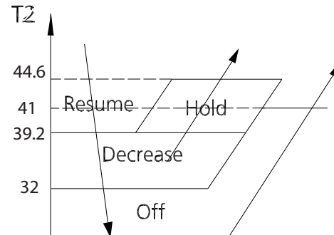
Fig. 20 —Evaporator Temperature Protection
