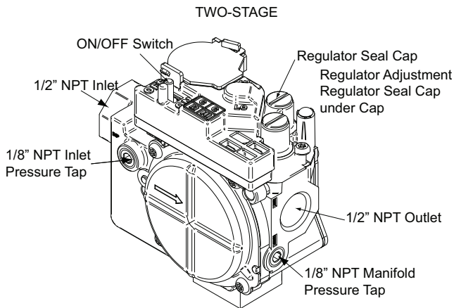
Fig. 53 - Gas Valve
