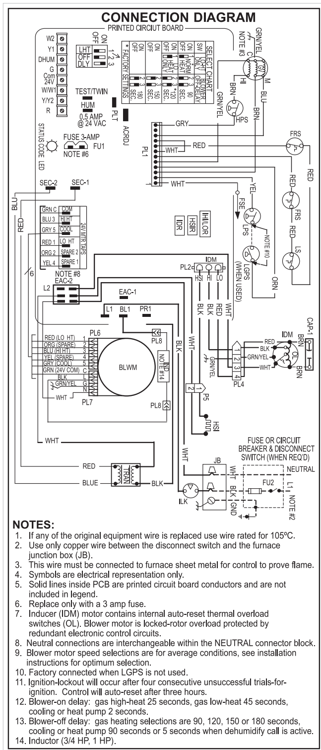
Fig. 65 - Wiring Diagram
