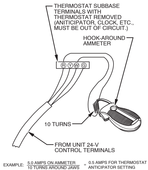
Fig. 55 - Amp. Draw Check with Ammeter
