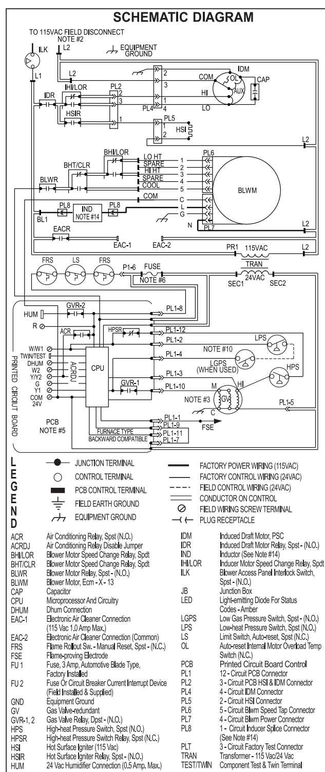
Fig. 65 - Wiring Diagram
