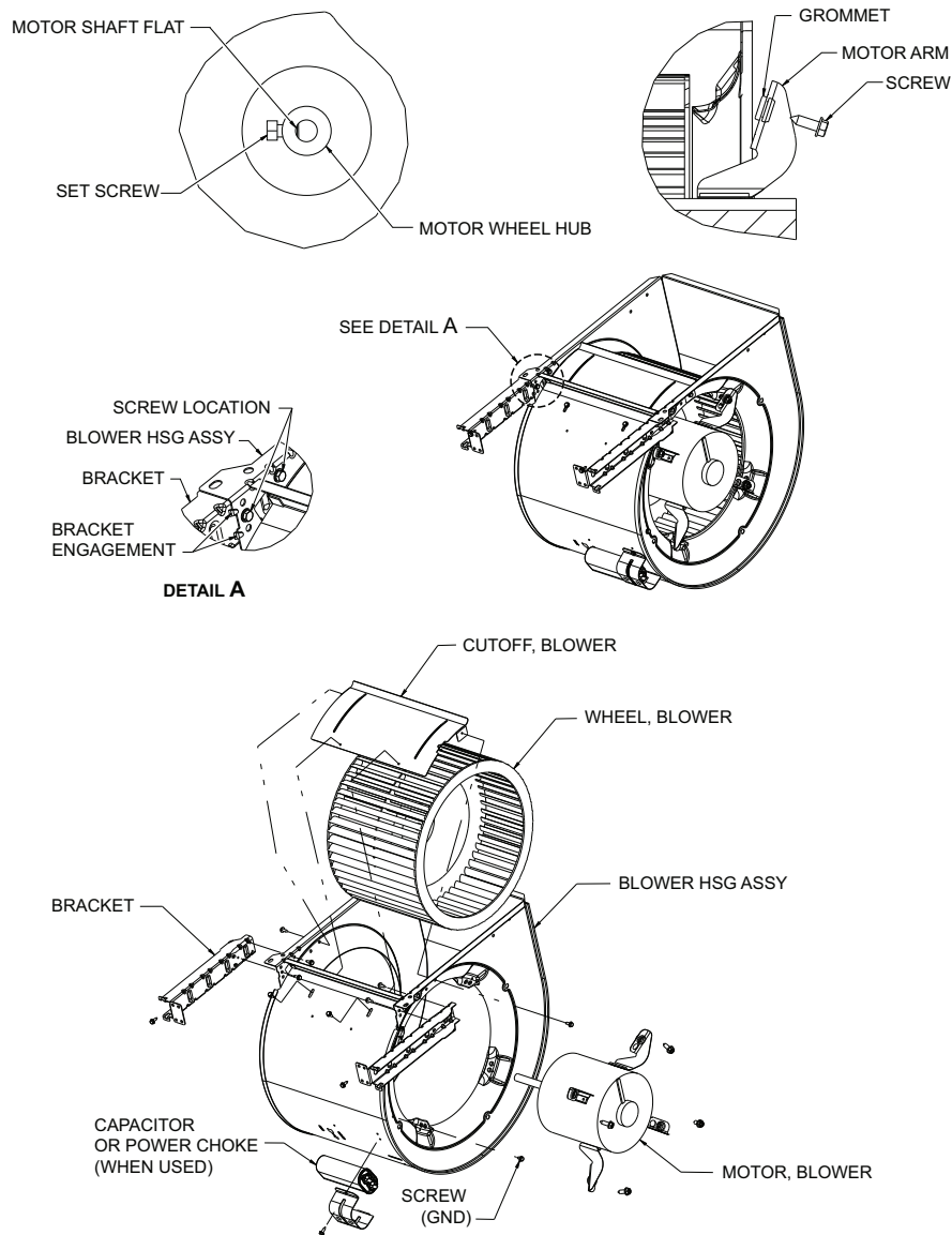
Fig. 62 - Blower Assembly
