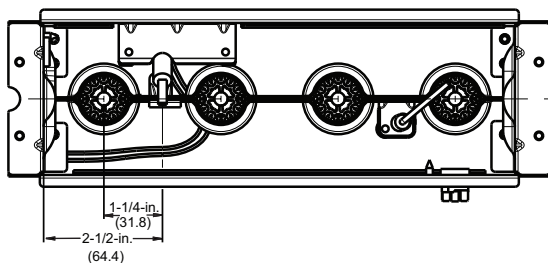
Fig. 57 - Igniter Position - Top View
