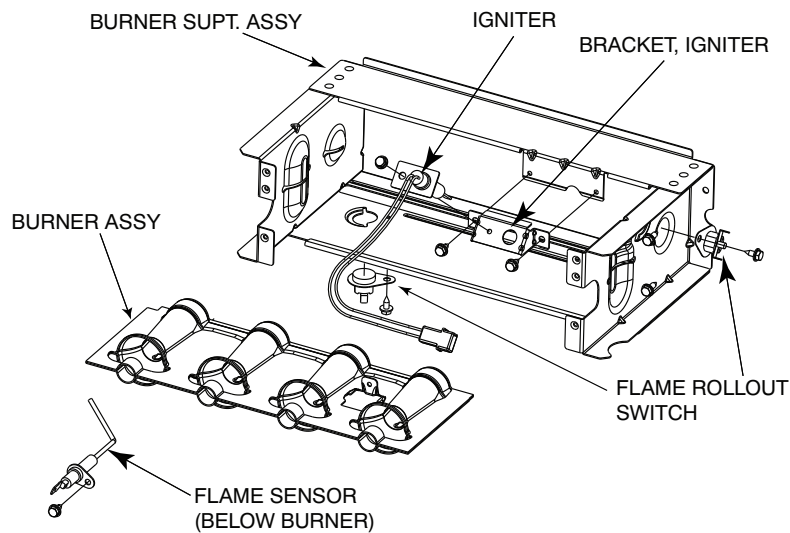
Fig. 63 - Burner Assembly
