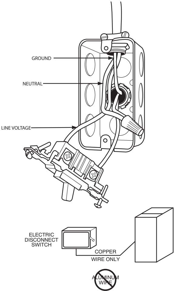
Fig. 32 - Field-Supplied Electrical Box on Furnace Casing
