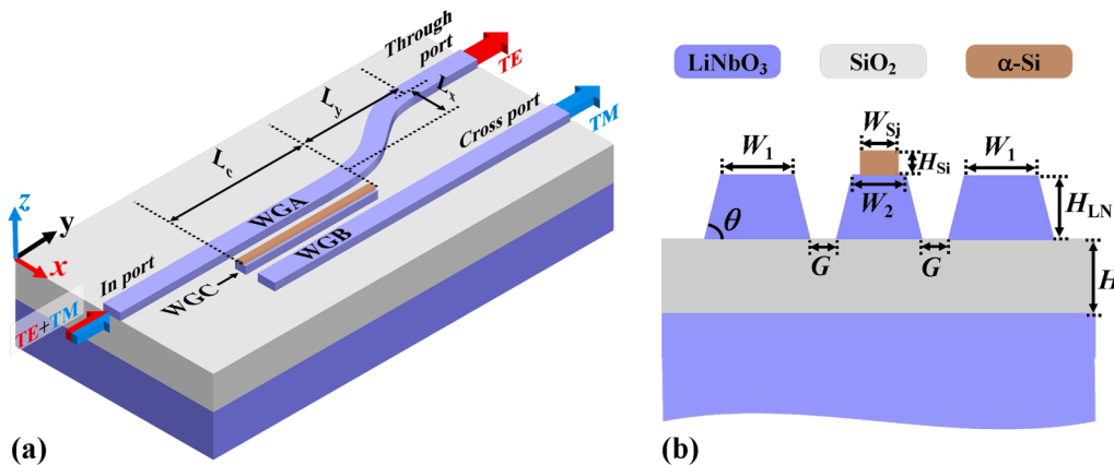
Fig. 1. Schematic diagram of proposed LNOI-based PBS. (a) 3D view and (b) cross-section view in the xz plane of the triple-waveguide coupler.
