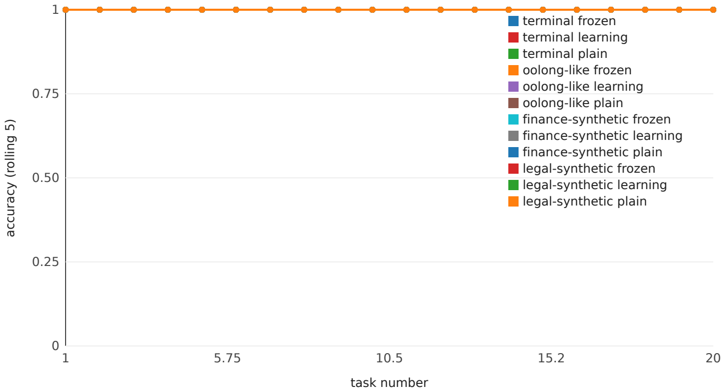
Learning curve
