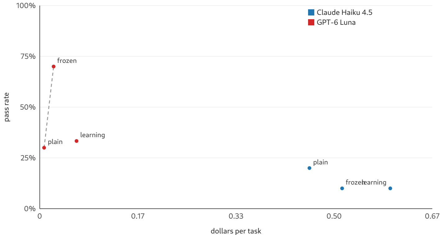
logbook-hard: pass rate against cost
