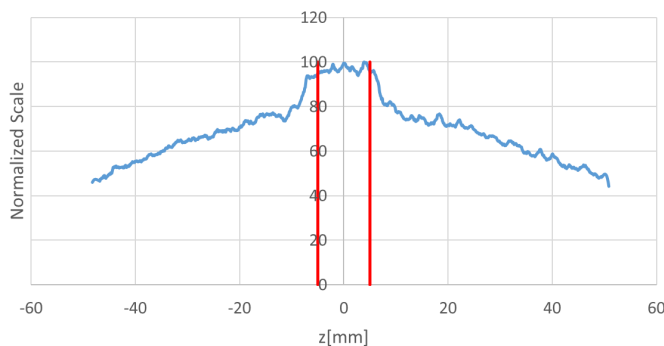
16x0.625, 16cm phantom, Head
