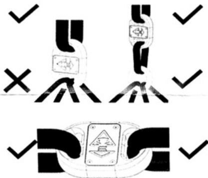
Figure 1 Incorrect and correct strop loading
