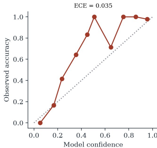
Figure 6.4 — Reliability Diagram of Final Confidence
