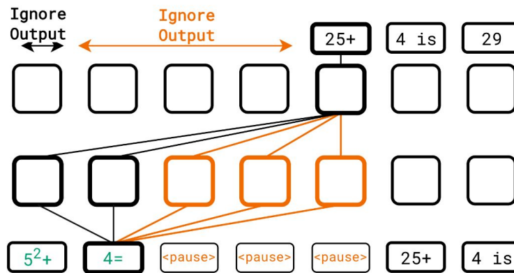
(b) Pause-inference and finetuning
