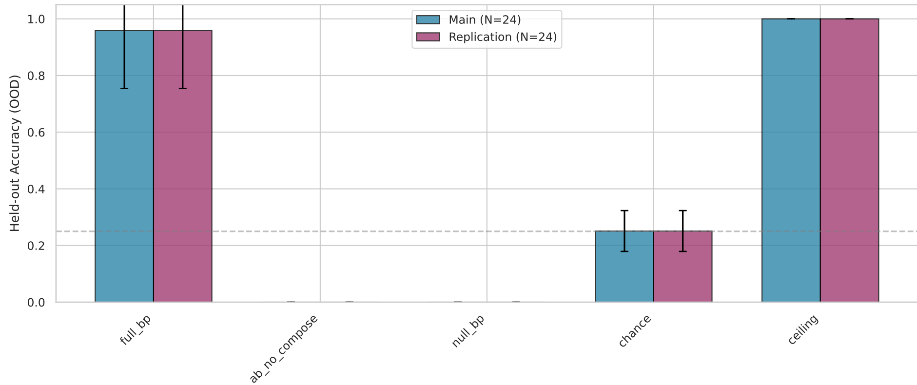
Phase 4: Structural-OOD Generalization (Held-out Triple)
