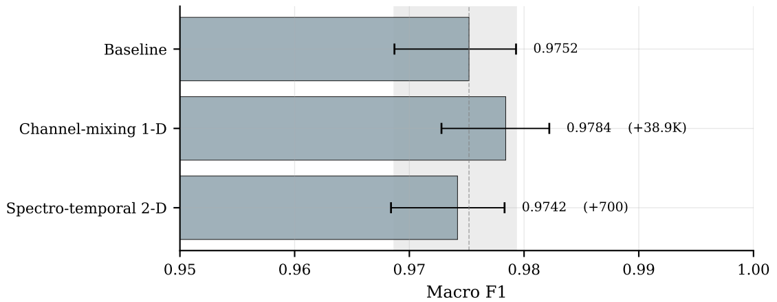
Figure 5.5: Learned-preprocessor scan.
