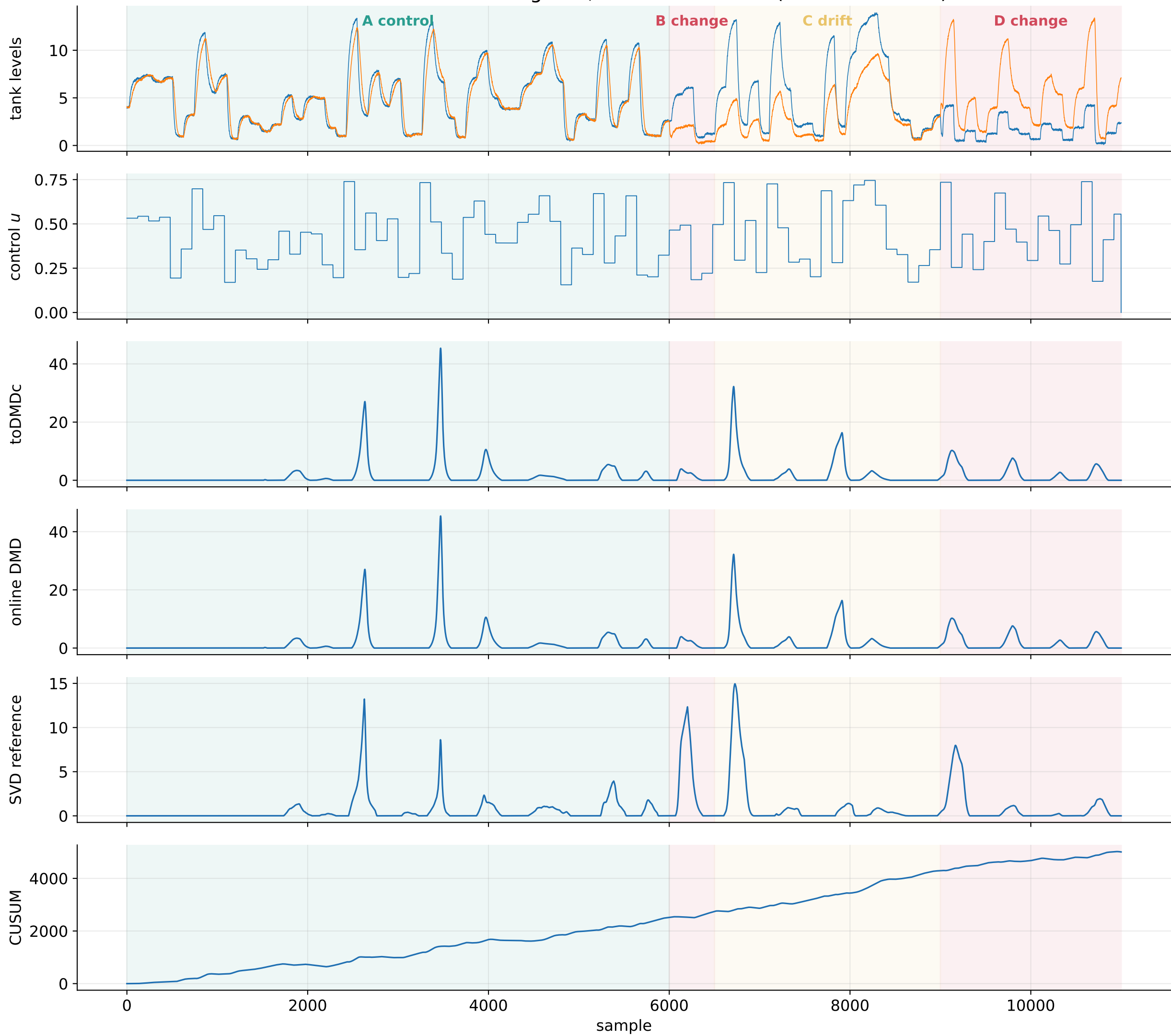
Two-tank: control throughout; faults in the MAP (valve constants)
