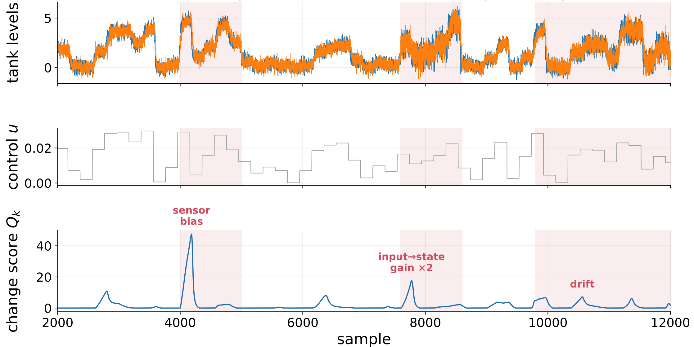
Nonlinear controlled plant — detects sensor bias, a gain change, and drift
