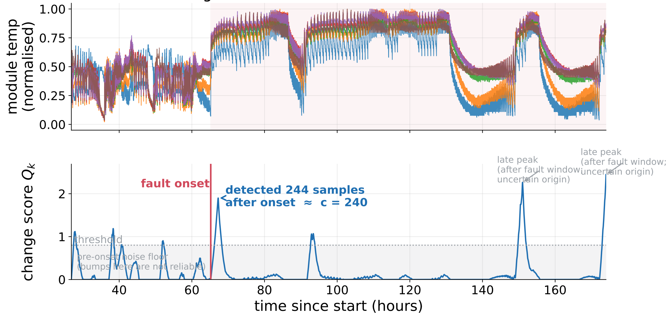
Real BESS cooling-fan fault — detected on data the model never saw
