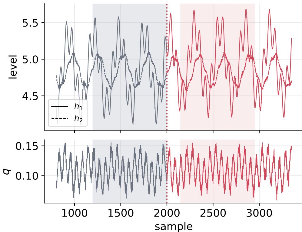
two-tank levels: valve k_1 clogs by 1 %
