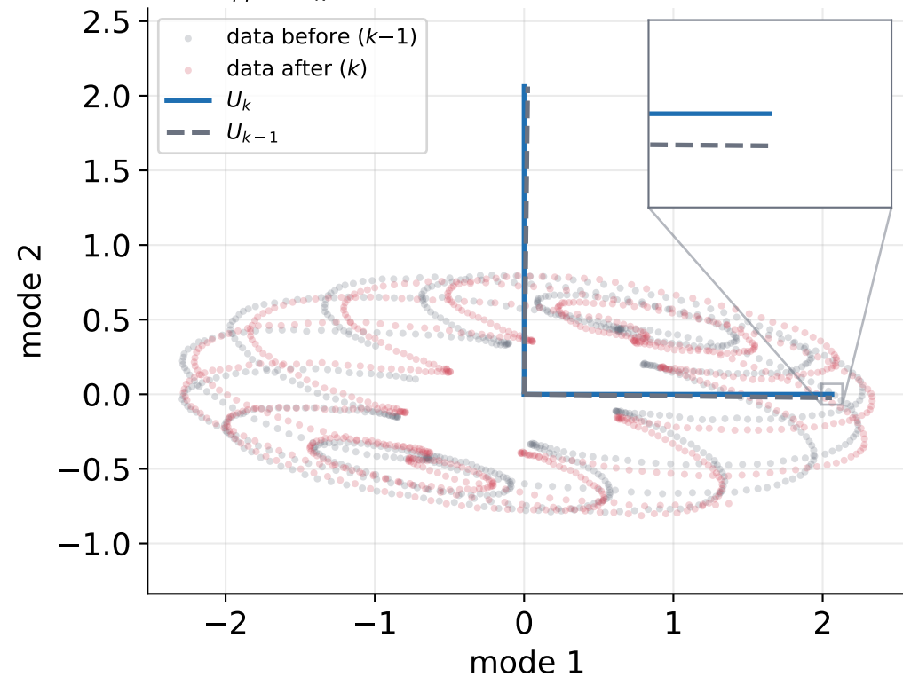
K_{pp} = U_k^\top U_{k-1} : basis rotates by \theta \approx -0.67^\circ
