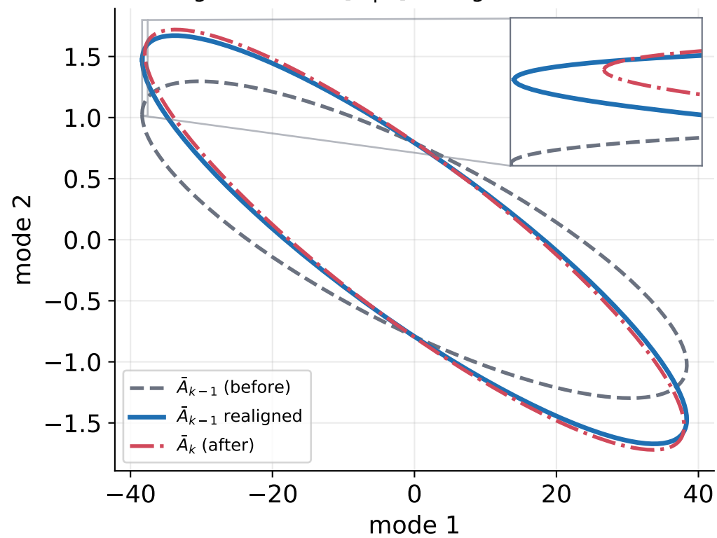
augmented \tilde{A} = [\tilde{A} \mid \tilde{B}] : realigned tracks after
