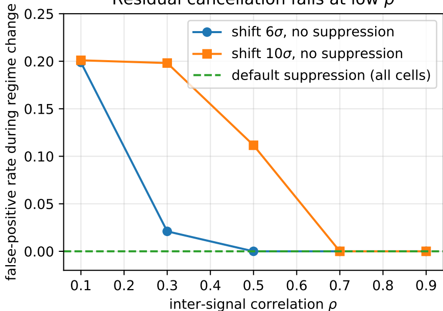
Residual cancellation fails at low \rho
