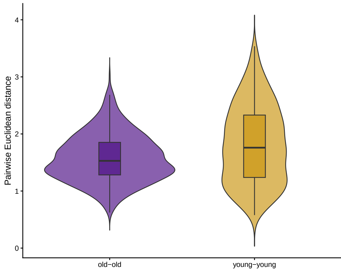
Within-group distances from DV genes: sn_only
