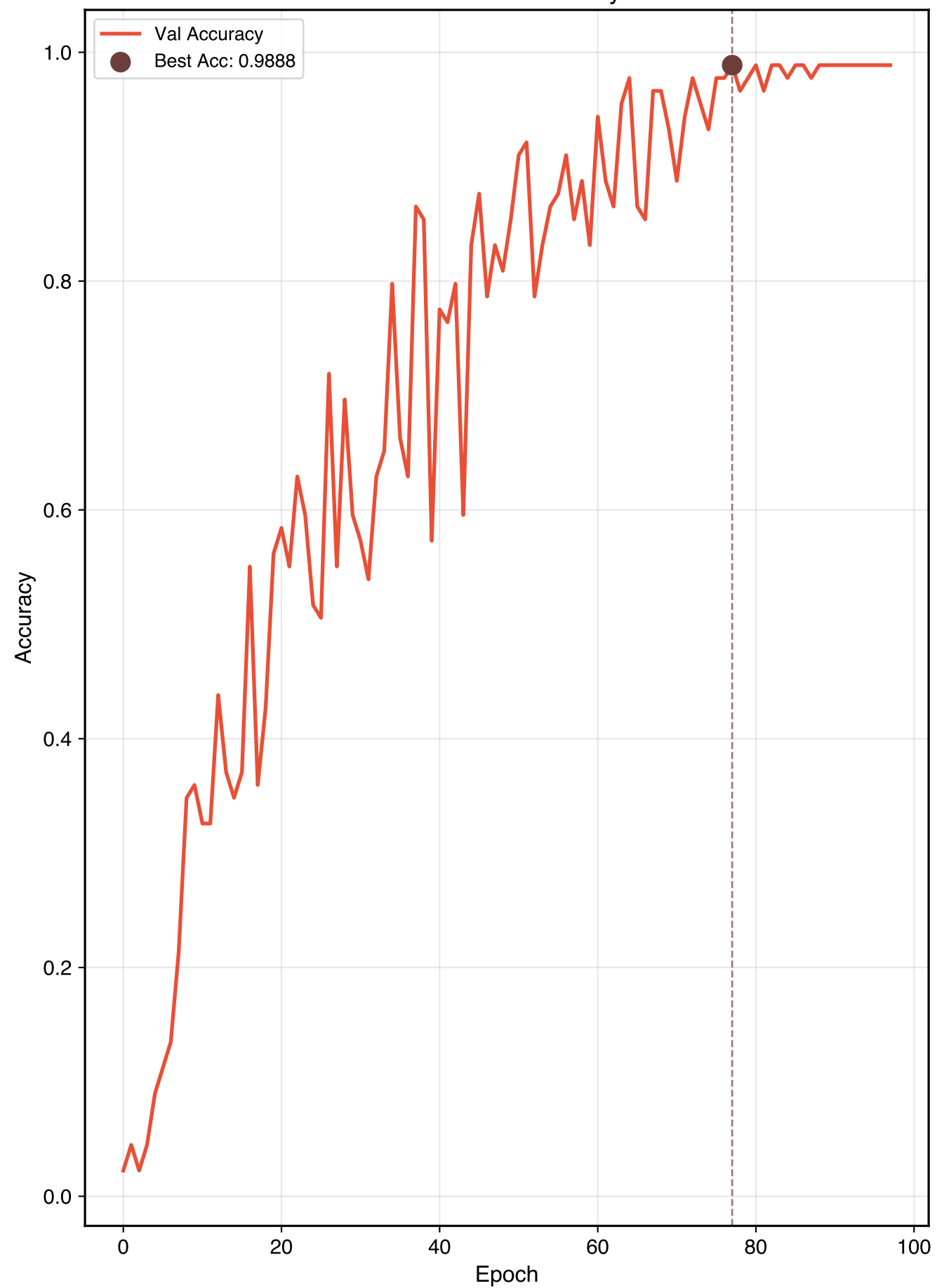
Validation Accuracy
