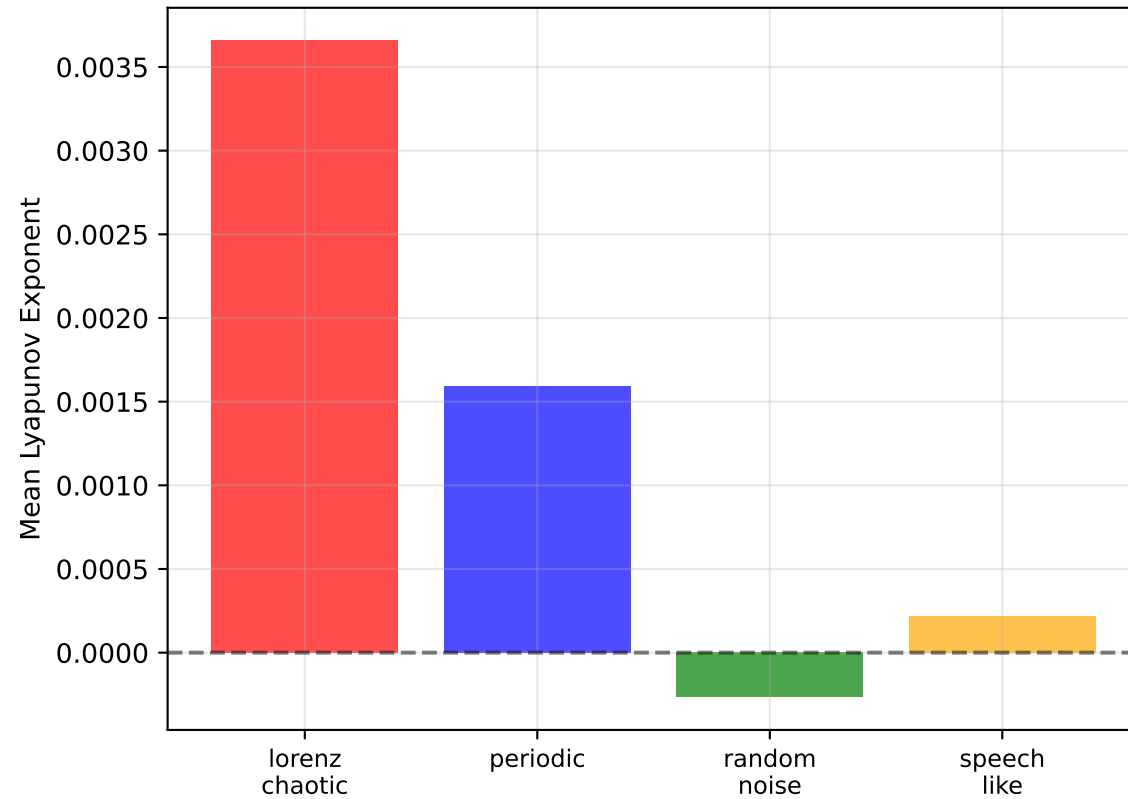
Exp 4: MLSA Robustness to Noise
