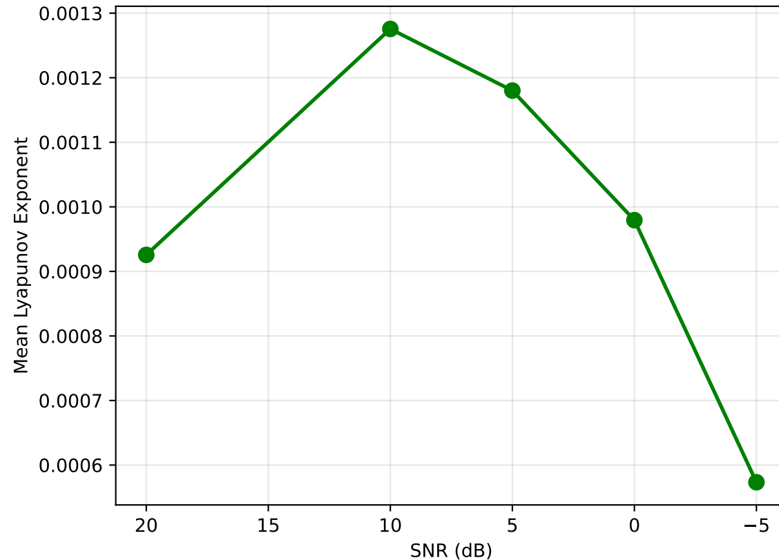
Exp 4: MLSA Robustness to Noise
