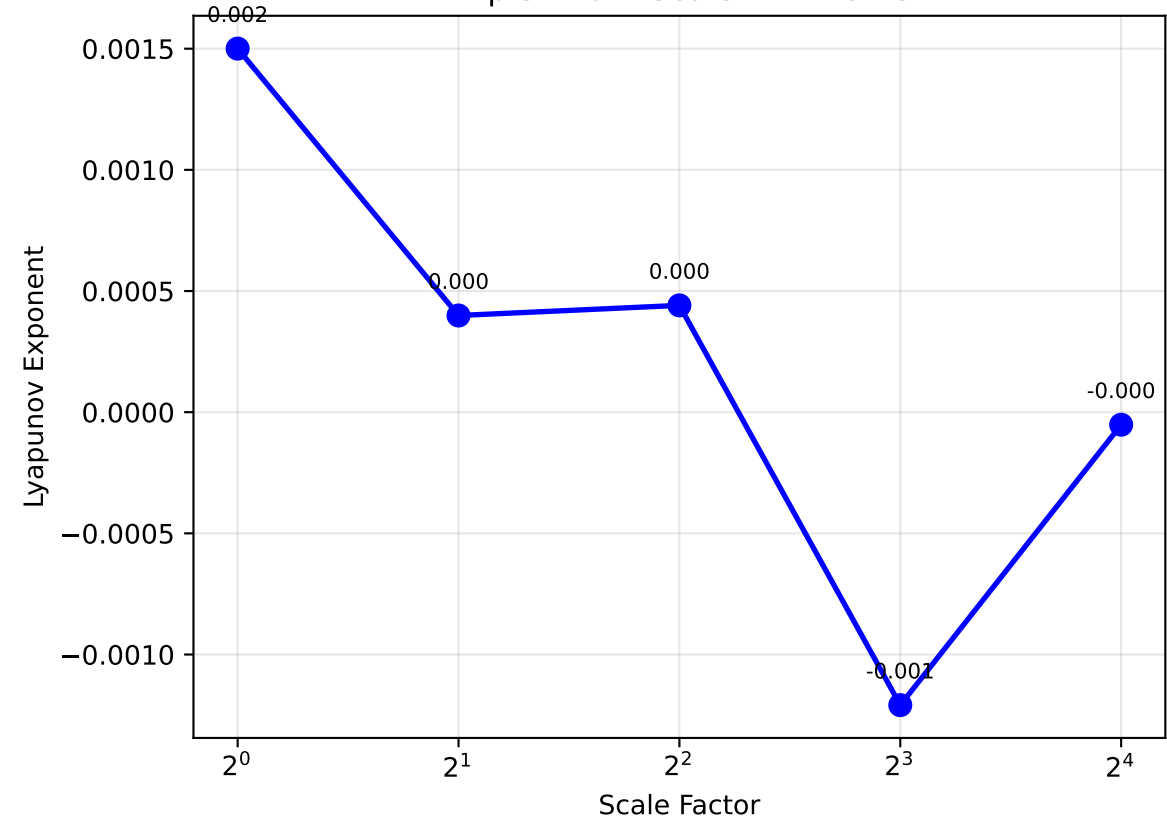
Exp 3: Multi-Scale LLE Profile
