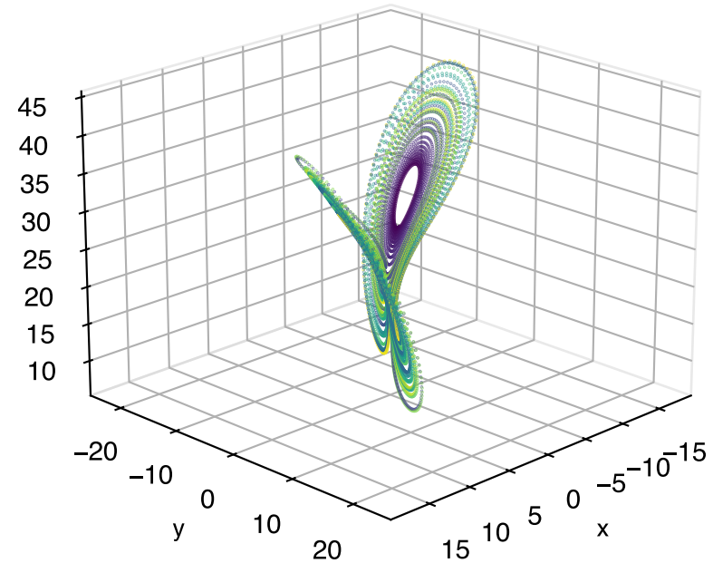
(a) Lorenz Attractor
