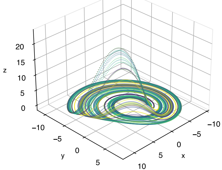
(b) Rössler Attractor
