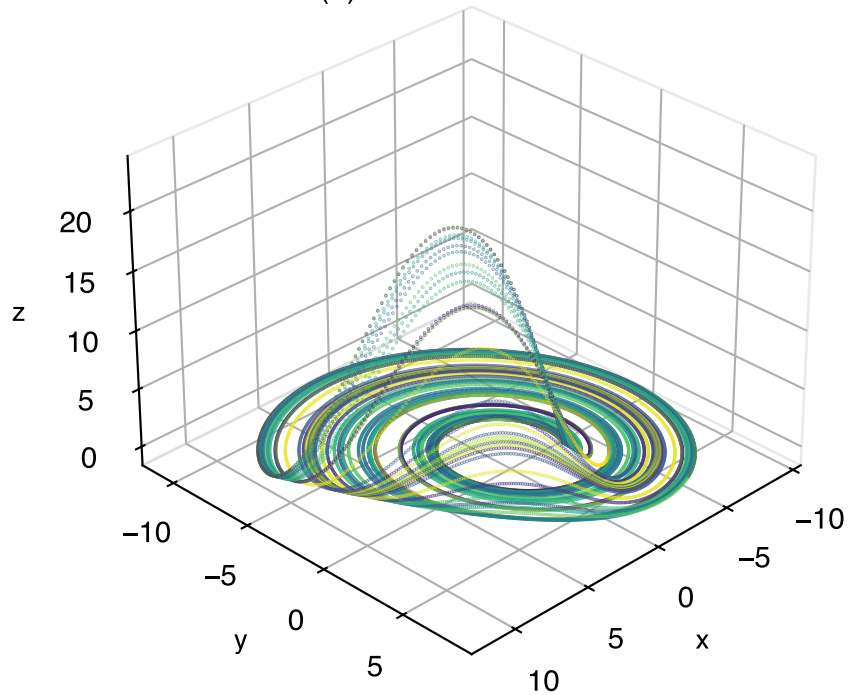
(b) Rössler Attractor
