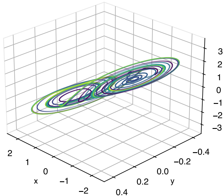
(b) Chua's Circuit Attractor
