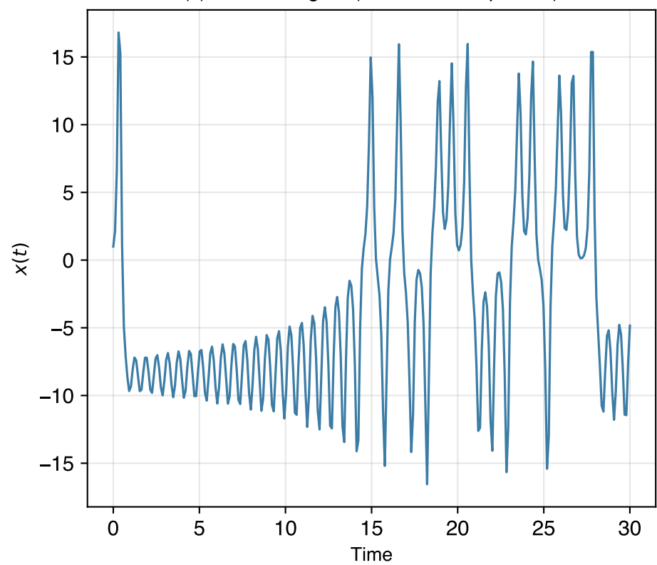
(c) Chaotic Signal (Lorenz x-component)
