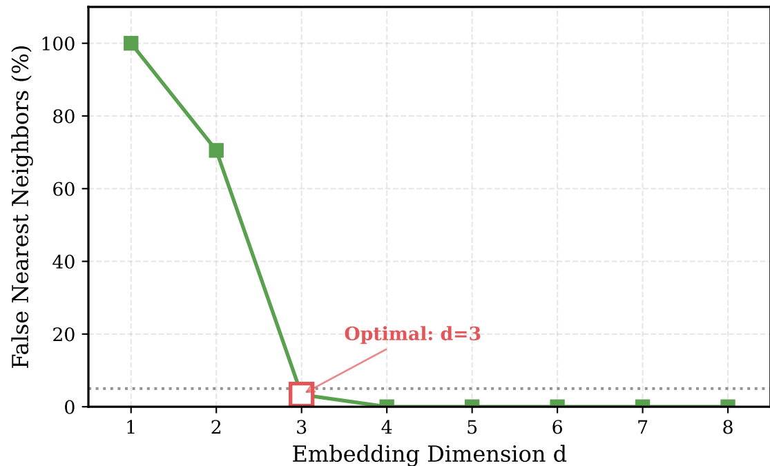
False Nearest Neighbors Analysis
