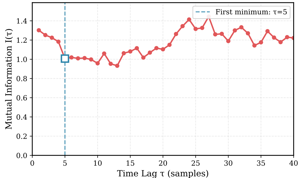
Mutual Information Function
