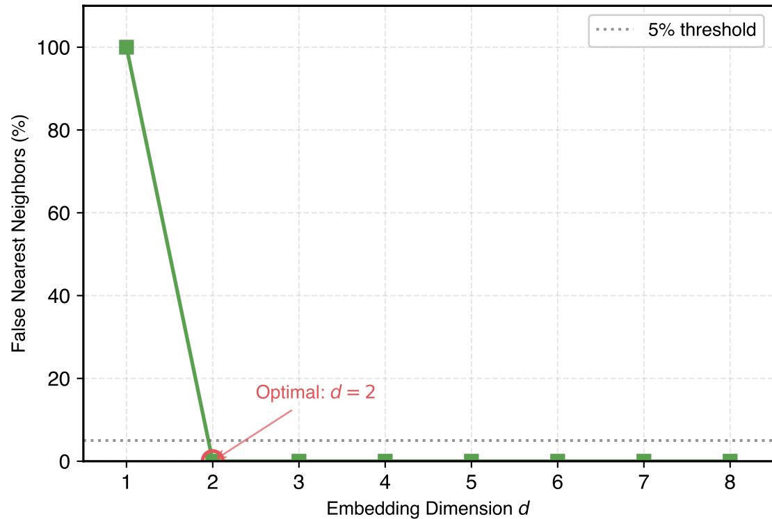
False Nearest Neighbors Analysis
