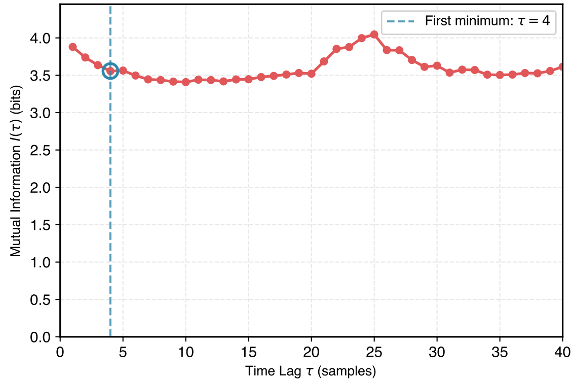
Mutual Information Function
