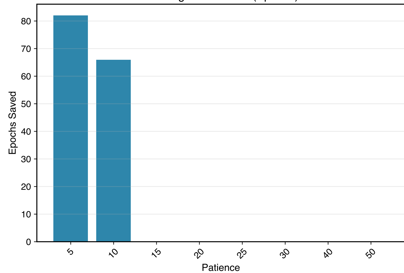
Training Time Saved (Epochs)
