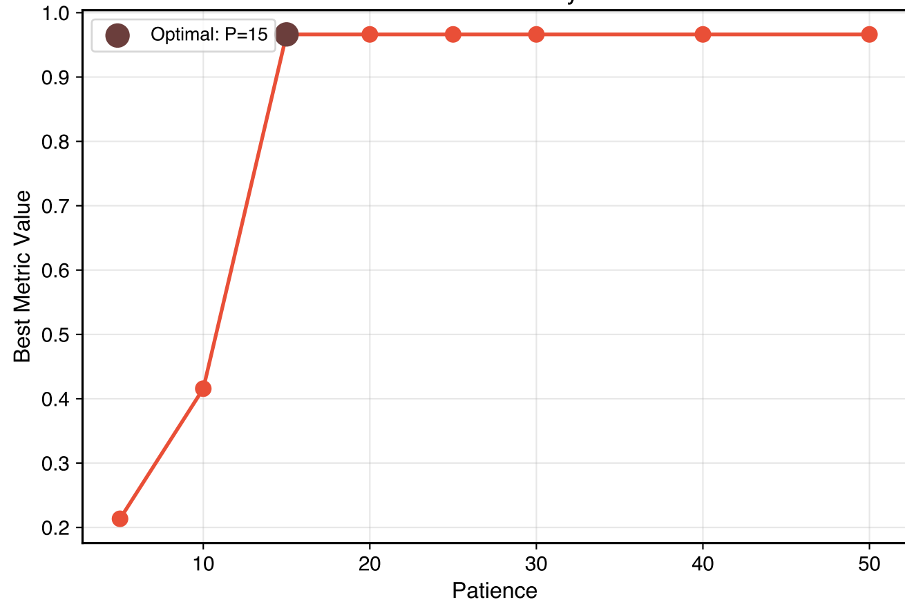
Best Metric Achieved by Patience
