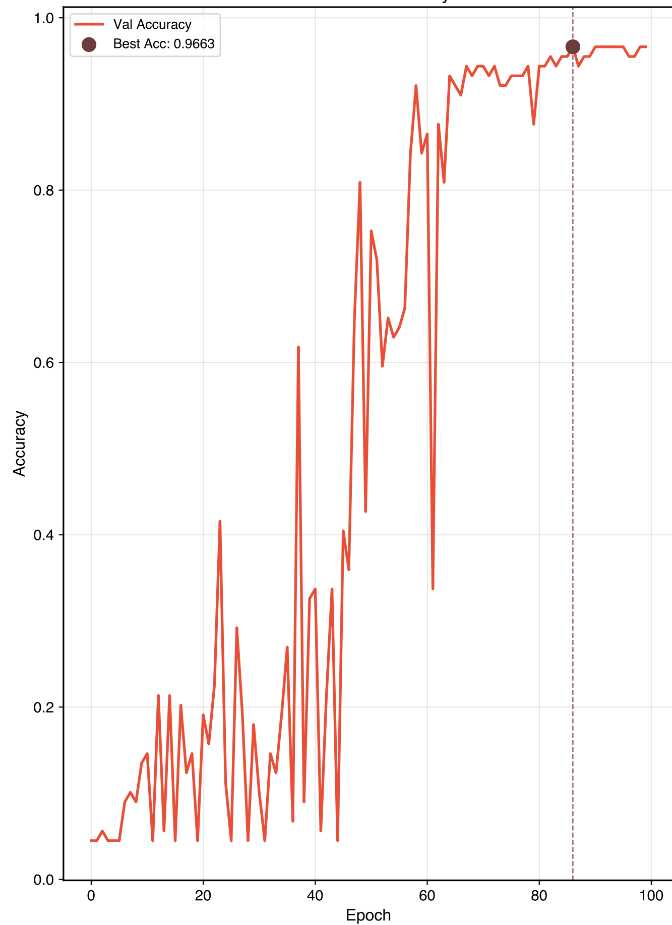
Validation Accuracy
