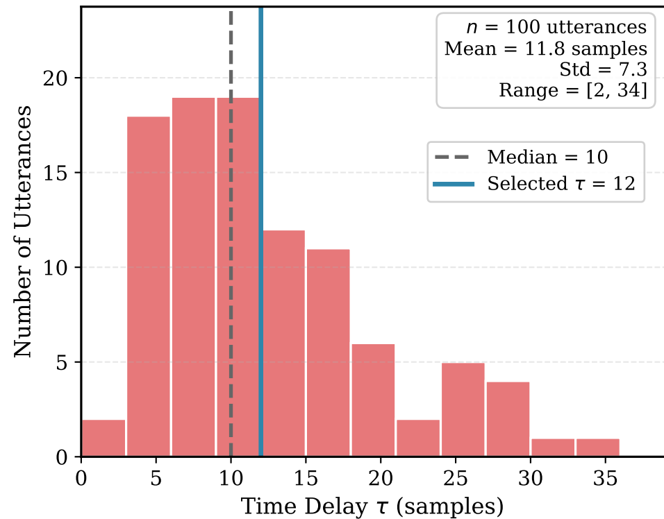
(a) Time Delay Distribution
