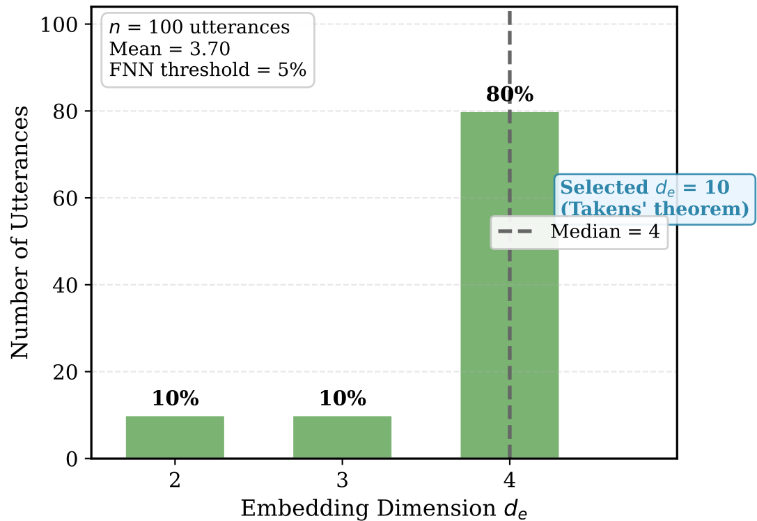
(b) Embedding Dimension Distribution
