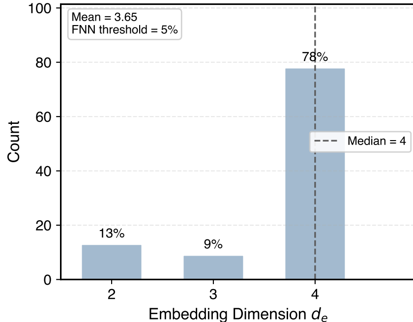
(b) Dimension Distribution
