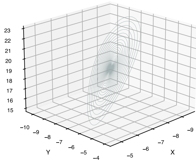
\rho=35.0 (Complex chaos)
