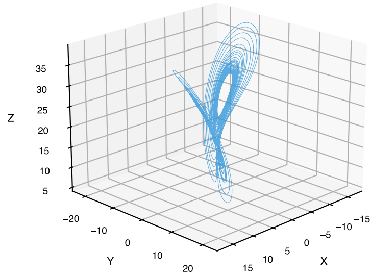
\rho=45.0 (High energy)
