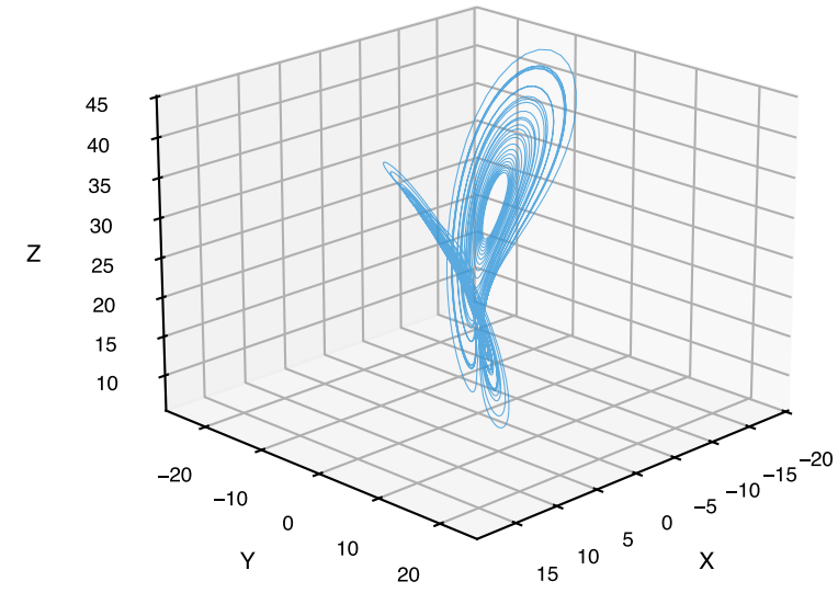
\rho=55.0 (Expanded attractor)
