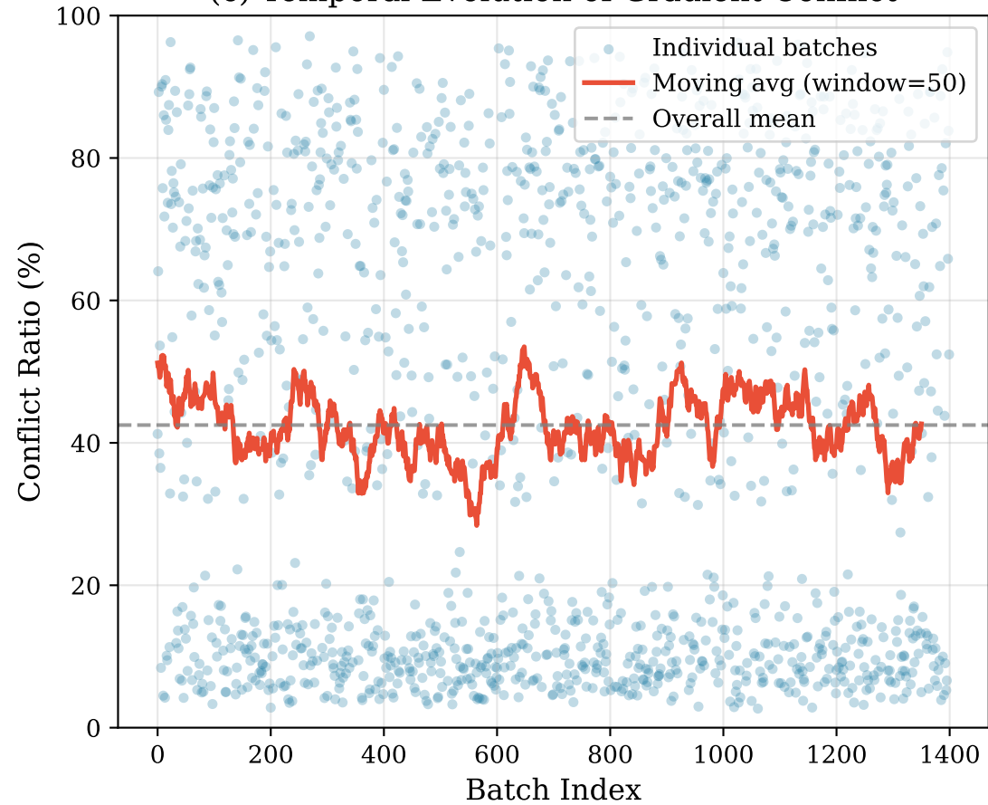
(c) Temporal Evolution of Gradient Conflict
