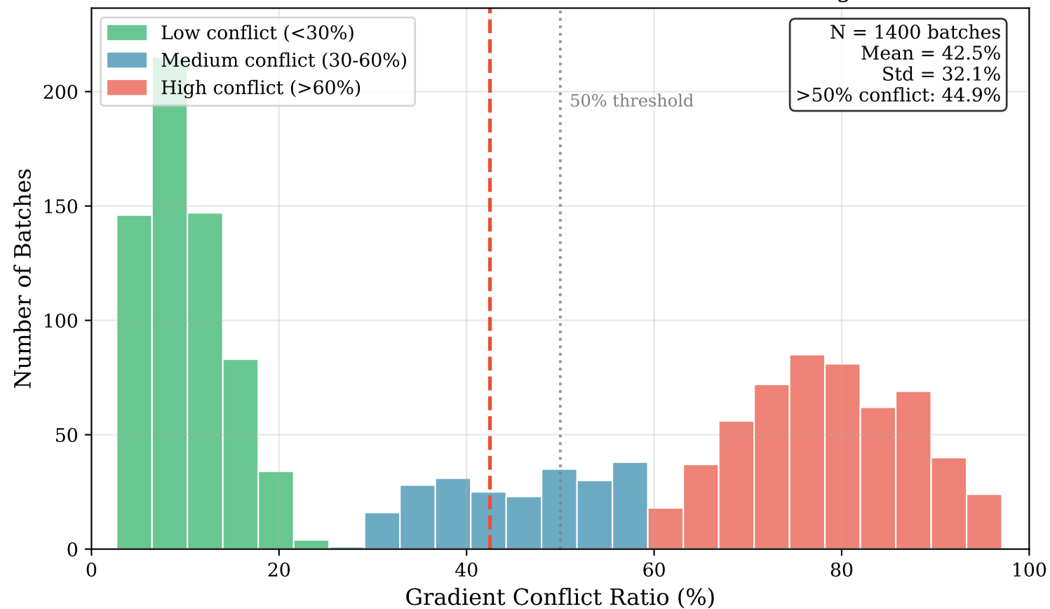
Distribution of Gradient Conflict Ratios Across Training Batches
