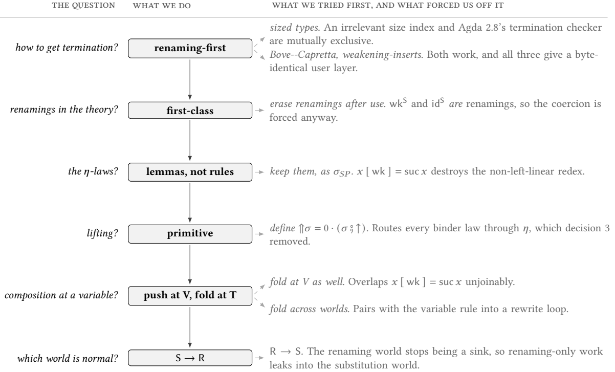
Figure 3. How the rule set was found. Only the first decision is a matter of taste. Every later one is forced, by a critical pair that will not join, a law that can be stated but not oriented, or a redex destroyed before its rule can fire.
