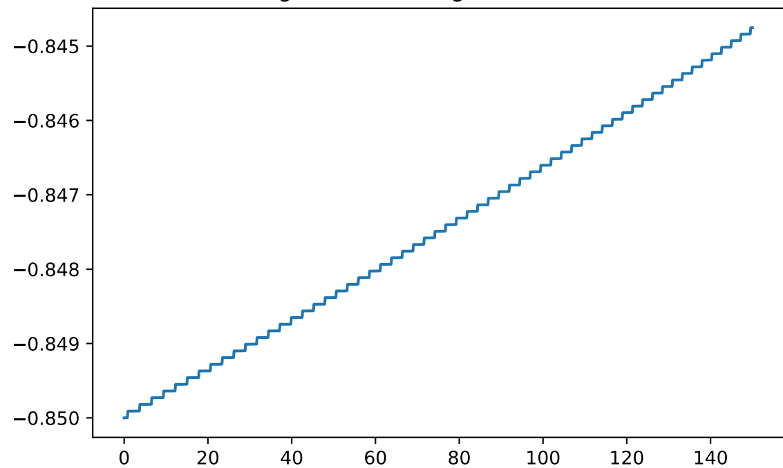
Runge-Kutta 3/8 Angular Momentum
