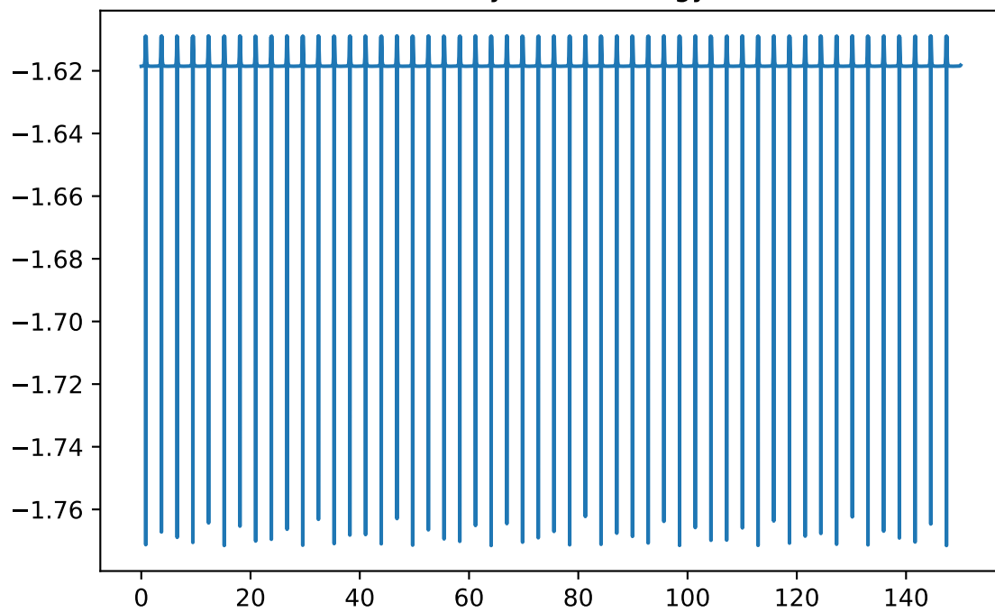
Velocity-Verlet Energy
