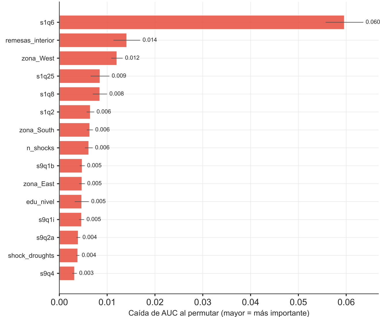
Permutation Importance – Random Forest (test set, 10 repeticiones)
