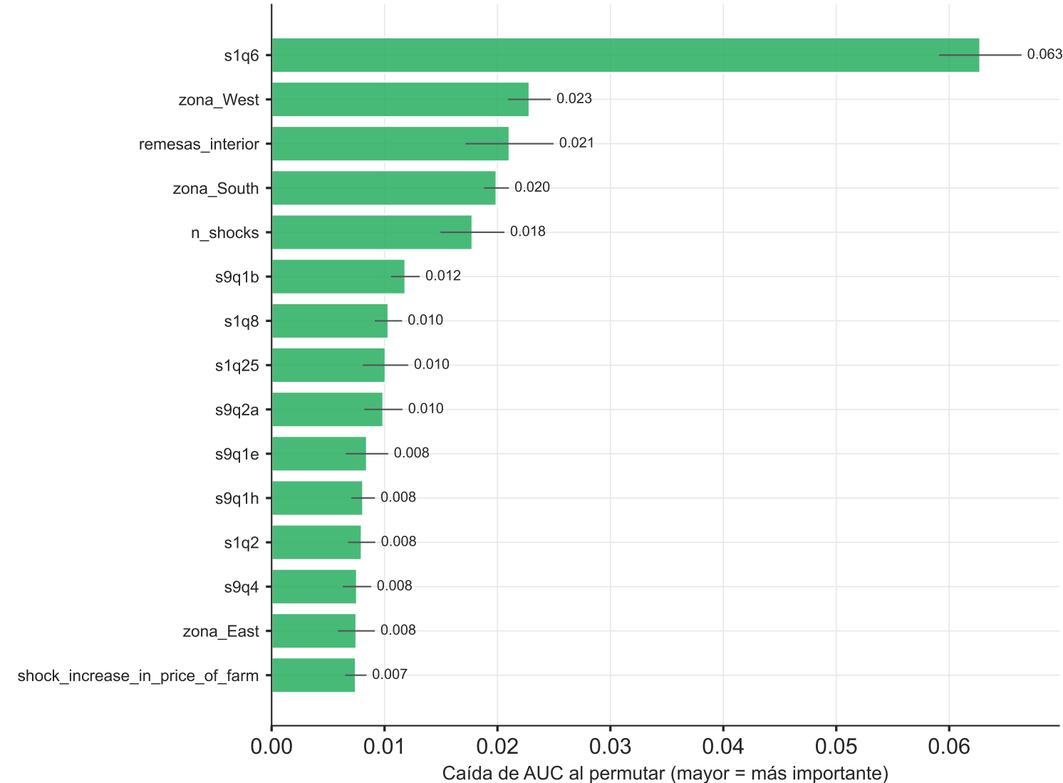
Permutation Importance – Gradient Boosting (test set, 10 repeticiones)
