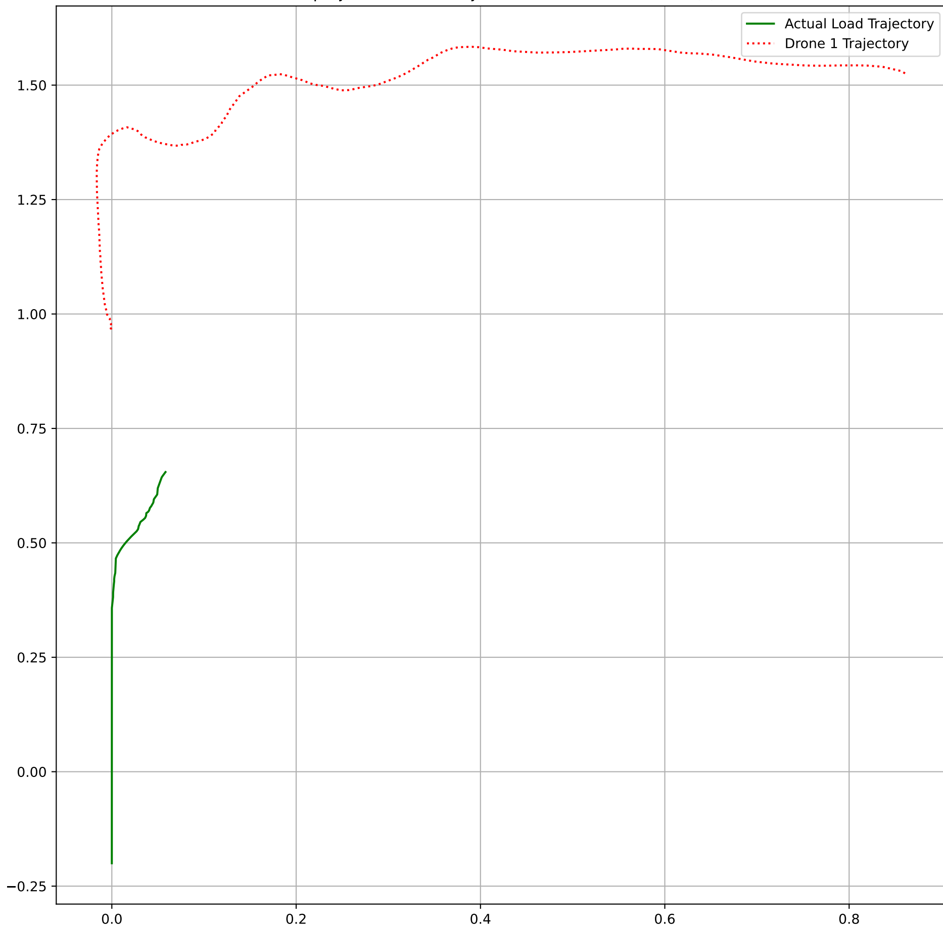
XY projection of 3D Trajectories of Load and Drone(s)
