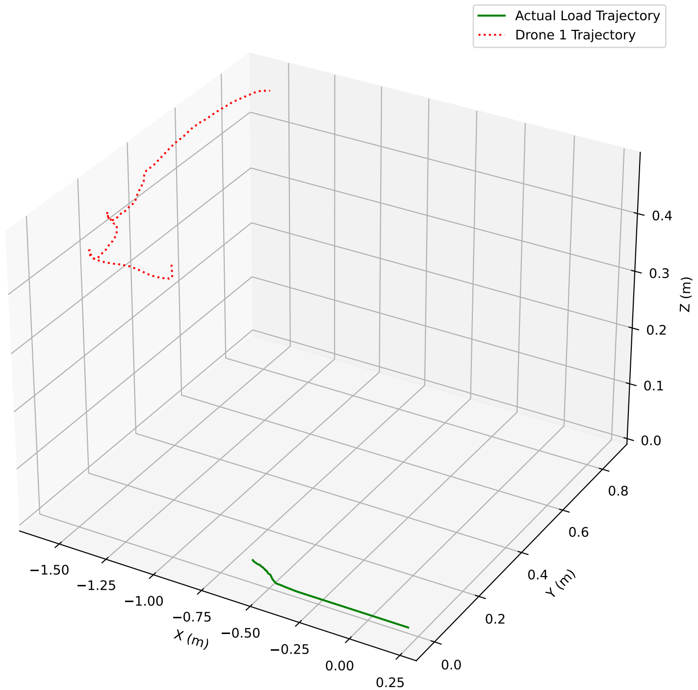
3D Trajectories of Load and Drone(s)
