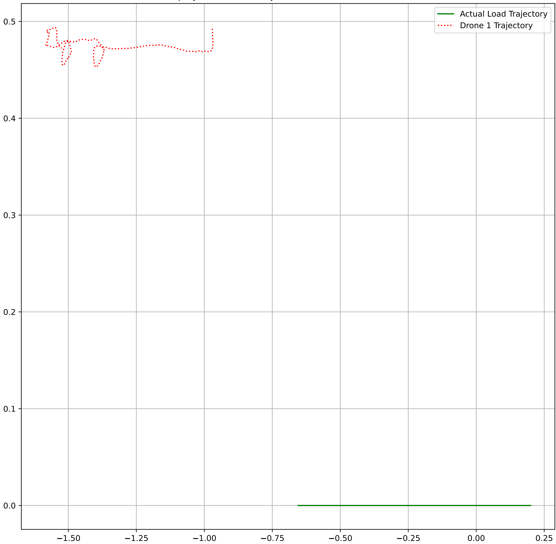
XZ projection of 3D Trajectories of Load and Drone(s)
