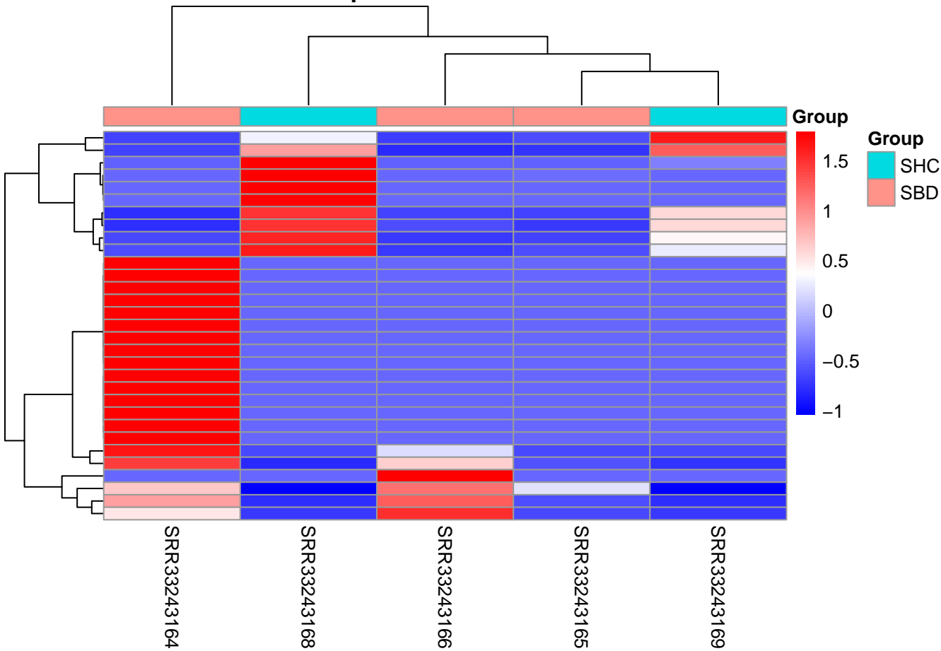
Heatmap of DEGs: SBD vs SHC
