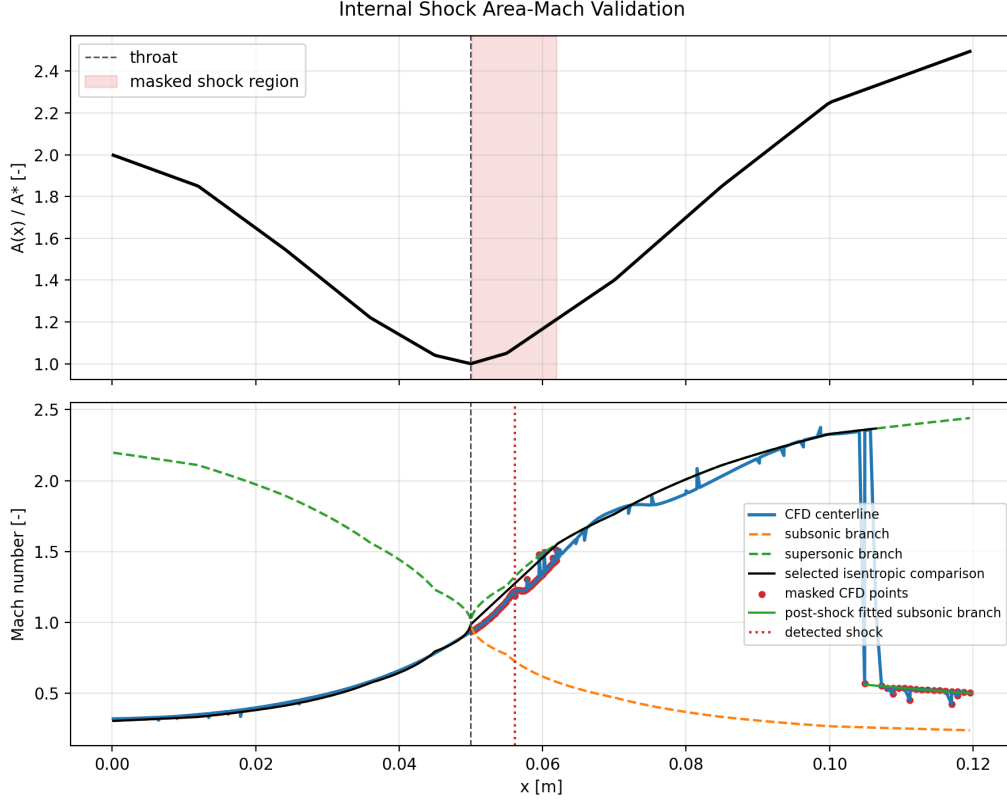
Figure 3: Internal-shock area-Mach validation. The shock region is masked and excluded from the isentropic comparison.
