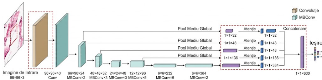
Figura 2.7: Schema unei arhitecturi EfficientNet-B3 [14]
