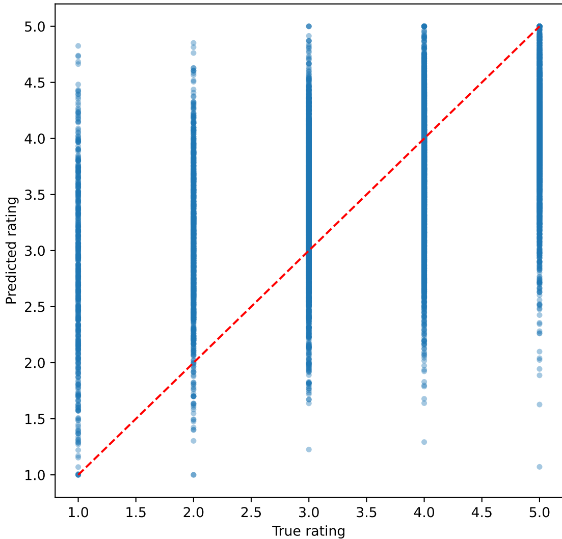
Scatter: RMSE=0.963, MAE=0.756
